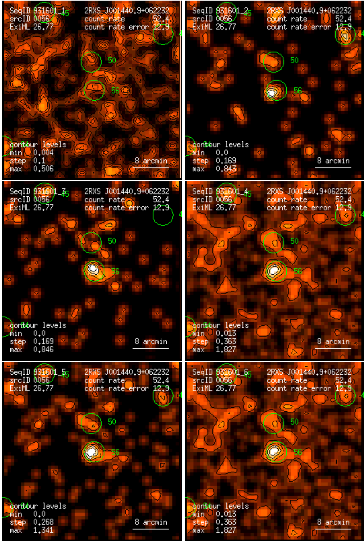
Figure 56: RASS 931601: detection 0056: band rate images, Gaussian filter: (1) PSPC channels 11 – 41, (2) 52 – 90, (3) 91 – 201, (4) 11 – 235, (5) 52 – 201, (6) 11 – 201. Broad band rates in counts/ks. Band rate contour levels in counts/ks/arcmin 2 .
