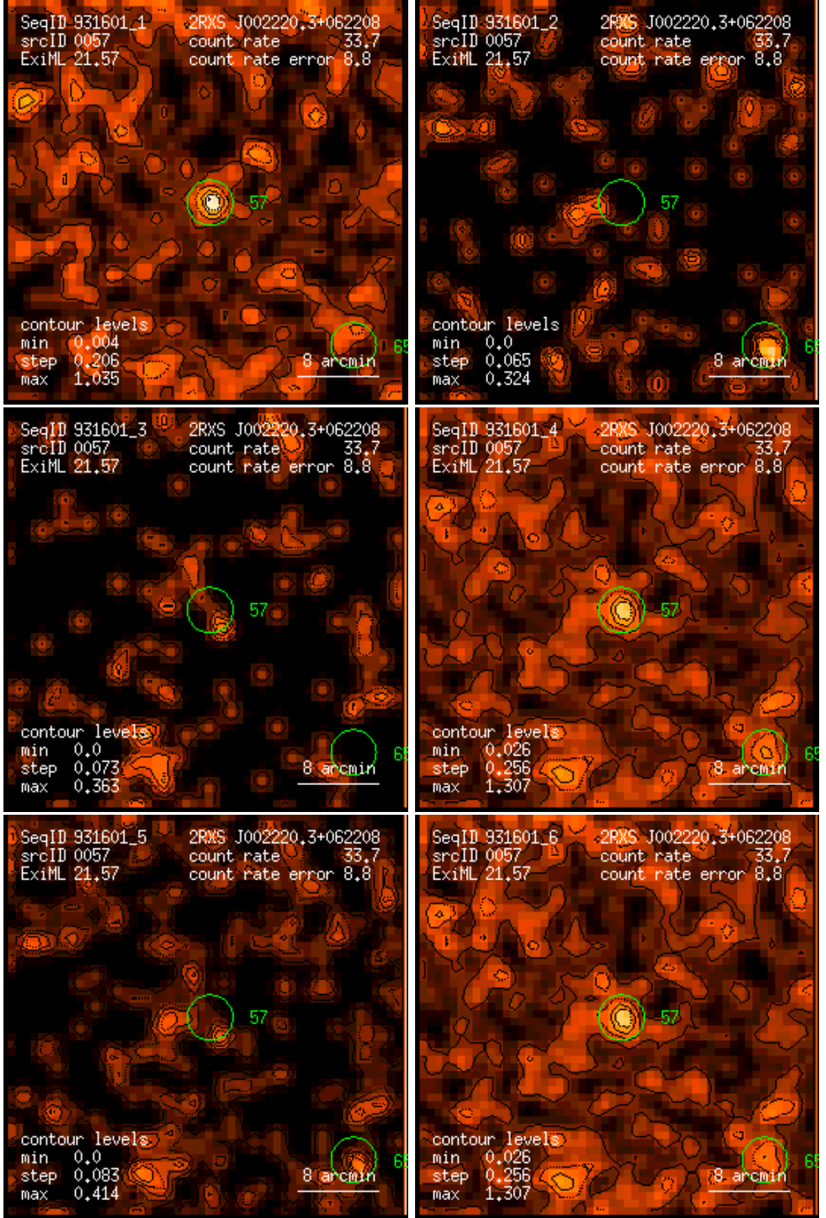
Figure 57: RASS 931601: detection 0057: band rate images, Gaussian filter: (1) PSPC channels 11 – 41, (2) 52 – 90, (3) 91 – 201, (4) 11 – 235, (5) 52 – 201, (6) 11 – 201. Broad band rates in counts/ks. Band rate contour levels in counts/ks/arcmin 2 .
