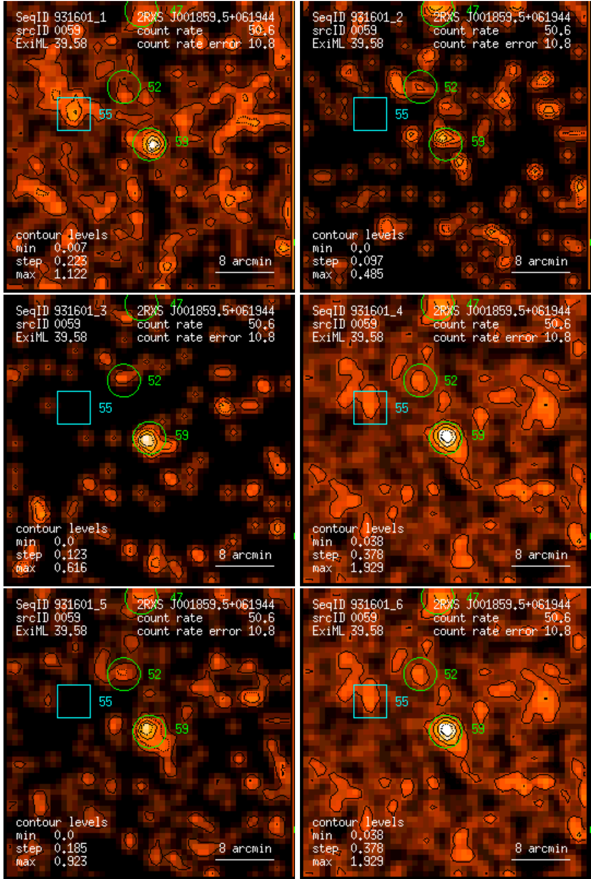
Figure 59: RASS 931601: detection 0059: band rate images, Gaussian filter: (1) PSPC channels 11 – 41, (2) 52 – 90, (3) 91 – 201, (4) 11 – 235, (5) 52 – 201, (6) 11 – 201. Broad band rates in counts/ks. Band rate contour levels in counts/ks/arcmin 2 .
