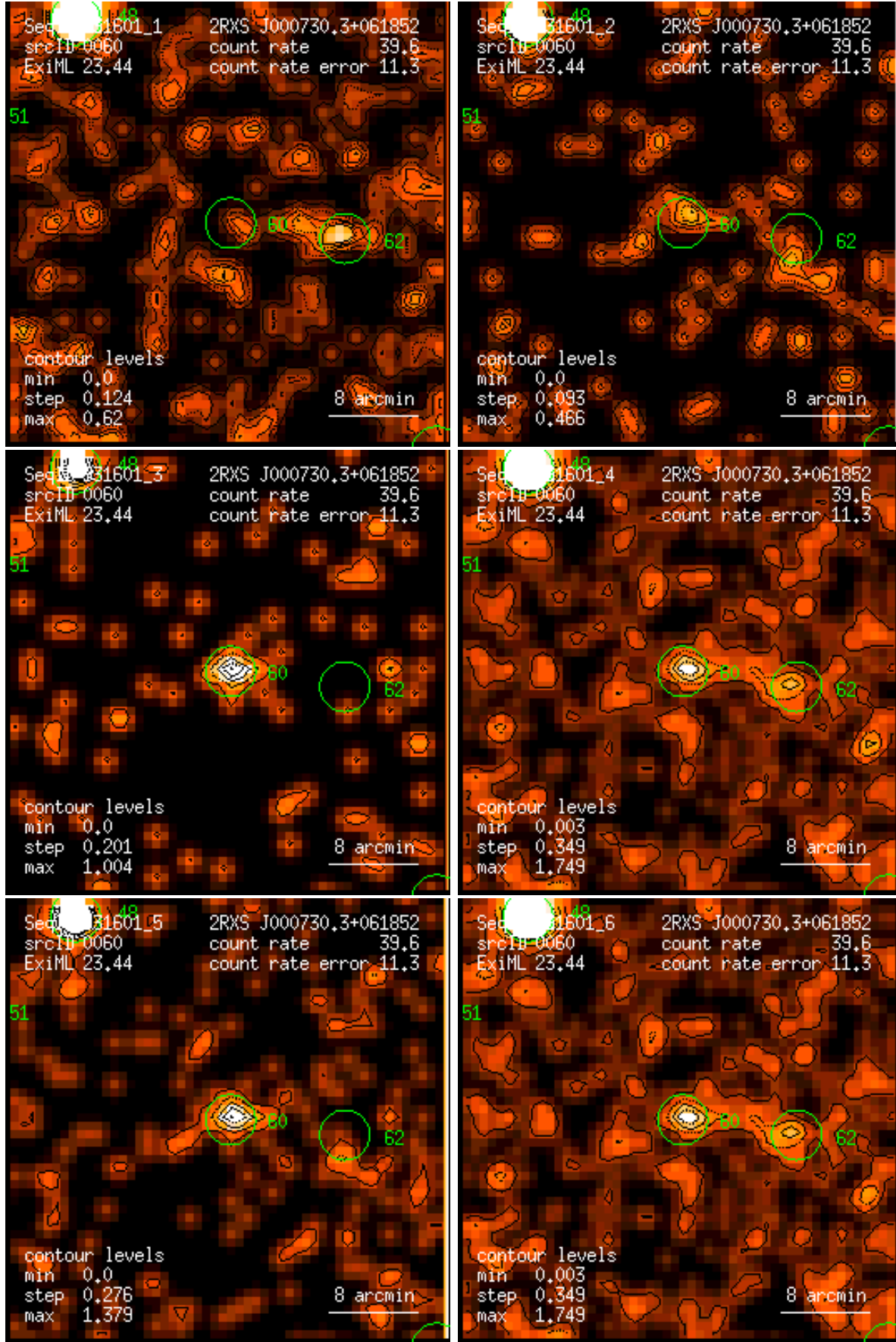
Figure 60: RASS 931601: detection 0060: band rate images, Gaussian filter: (1) PSPC channels 11 – 41, (2) 52 – 90, (3) 91 – 201, (4) 11 – 235, (5) 52 – 201, (6) 11 – 201. Broad band rates in counts/ks. Band rate contour levels in counts/ks/arcmin 2 .
