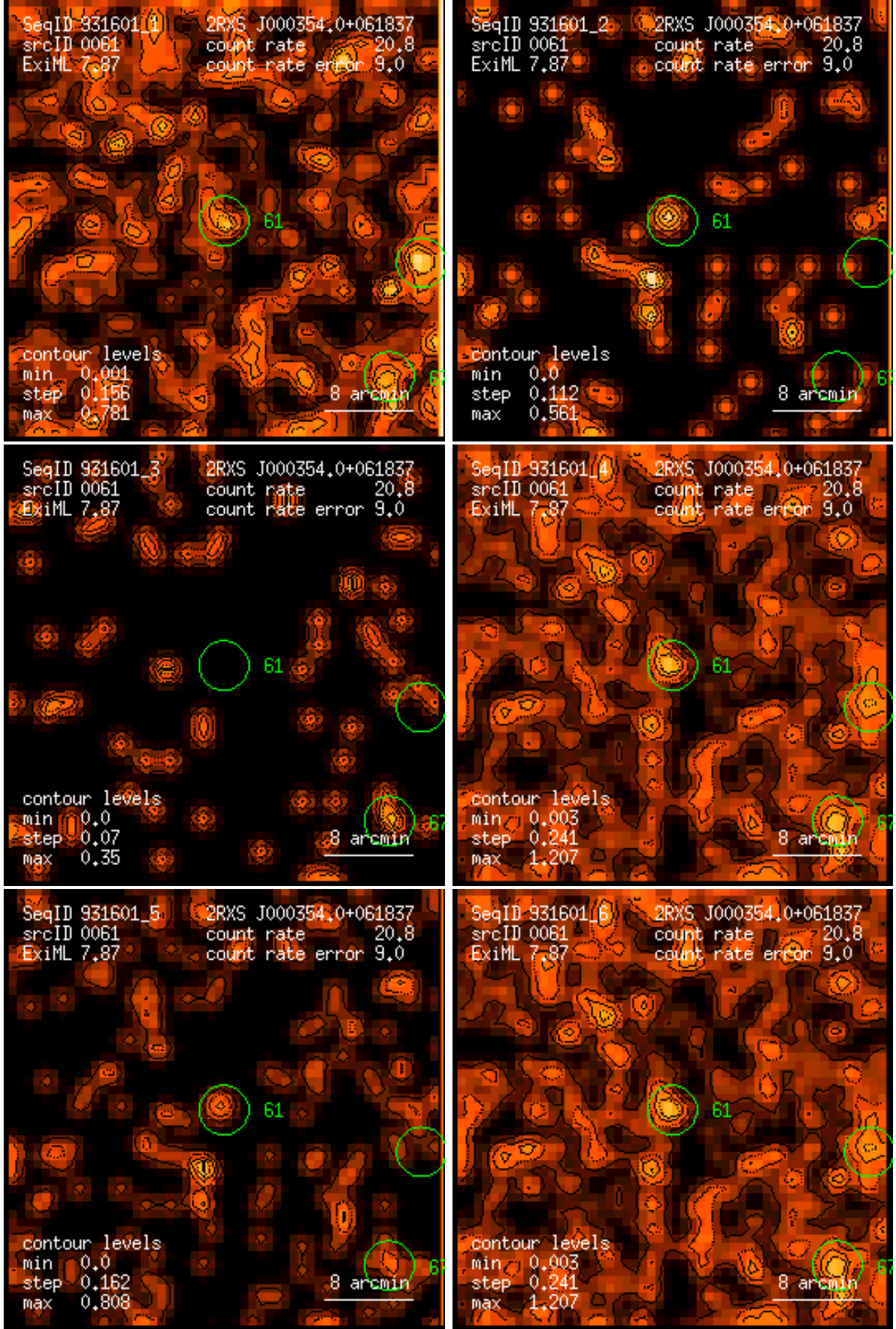
Figure 61: RASS 931601: detection 0061: band rate images, Gaussian filter: (1) PSPC channels 11 – 41, (2) 52 – 90, (3) 91 – 201, (4) 11 – 235, (5) 52 – 201, (6) 11 – 201. Broad band rates in counts/ks. Band rate contour levels in counts/ks/arcmin 2 .
