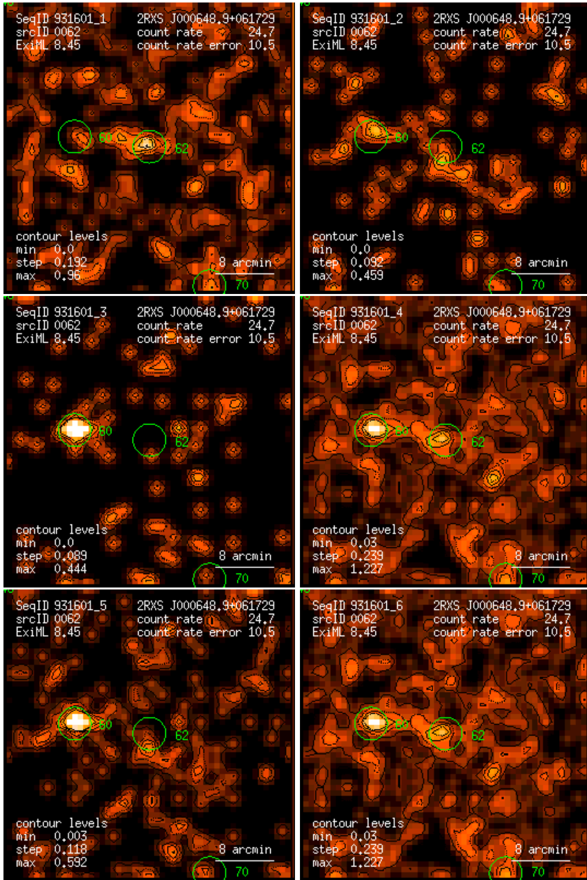
Figure 62: RASS 931601: detection 0062: band rate images, Gaussian filter: (1) PSPC channels 11 – 41, (2) 52 – 90, (3) 91 – 201, (4) 11 – 235, (5) 52 – 201, (6) 11 – 201. Broad band rates in counts/ks. Band rate contour levels in counts/ks/arcmin 2 .
