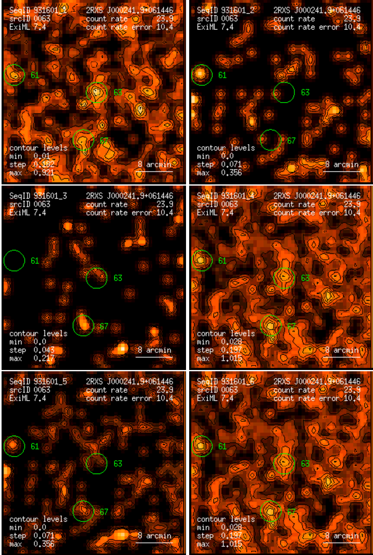
Figure 63: RASS 931601: detection 0063: band rate images, Gaussian filter: (1) PSPC channels 11 – 41, (2) 52 – 90, (3) 91 – 201, (4) 11 – 235, (5) 52 – 201, (6) 11 – 201. Broad band rates in counts/ks. Band rate contour levels in counts/ks/arcmin 2 .
