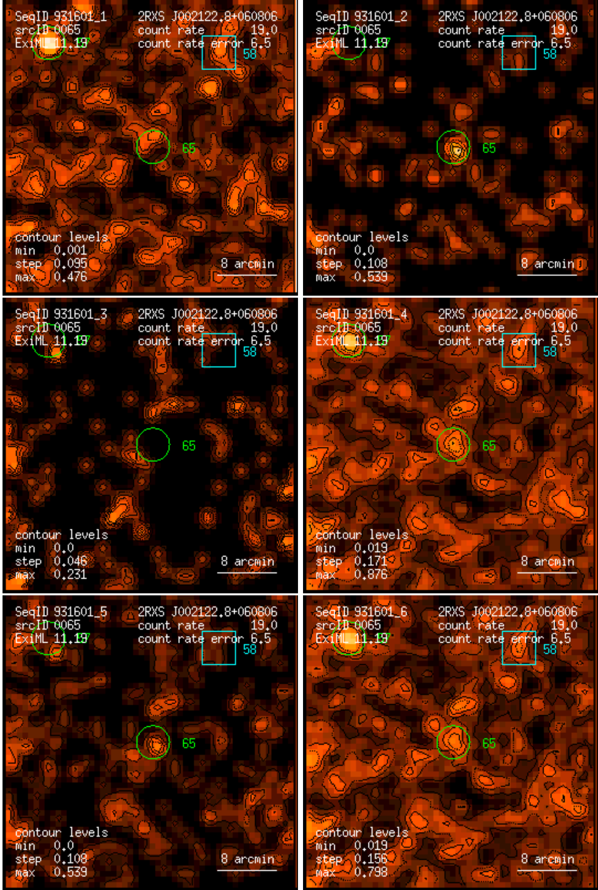
Figure 65: RASS 931601: detection 0065: band rate images, Gaussian filter: (1) PSPC channels 11 – 41, (2) 52 – 90, (3) 91 – 201, (4) 11 – 235, (5) 52 – 201, (6) 11 – 201. Broad band rates in counts/ks. Band rate contour levels in counts/ks/arcmin 2 .
