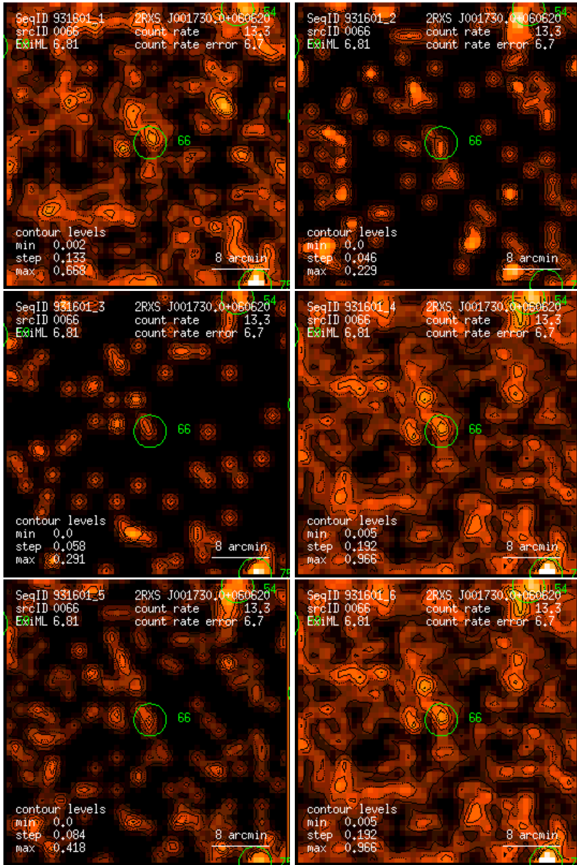
Figure 66: RASS 931601: detection 0066: band rate images, Gaussian filter: (1) PSPC channels 11 – 41, (2) 52 – 90, (3) 91 – 201, (4) 11 – 235, (5) 52 – 201, (6) 11 – 201. Broad band rates in counts/ks. Band rate contour levels in counts/ks/arcmin 2 .
