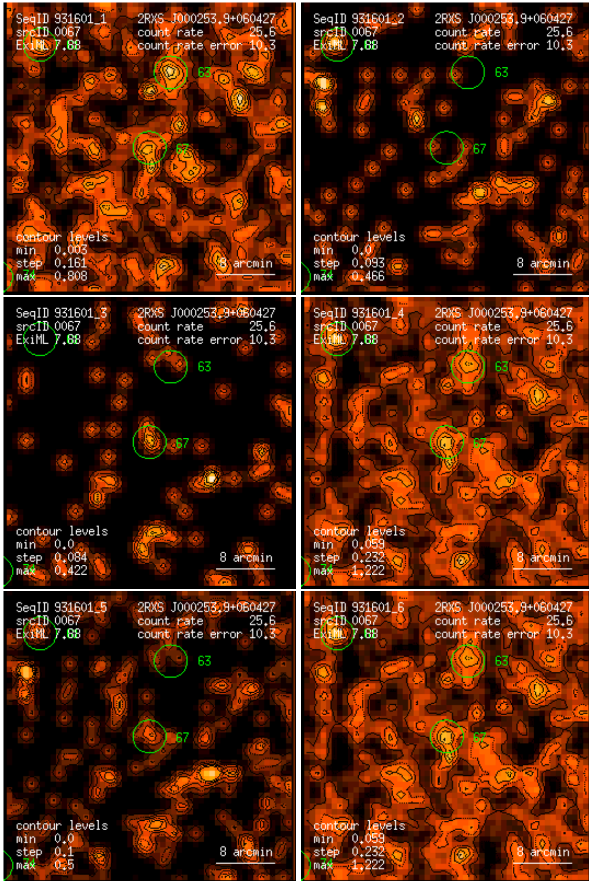
Figure 67: RASS 931601: detection 0067: band rate images, Gaussian filter: (1) PSPC channels 11 – 41, (2) 52 – 90, (3) 91 – 201, (4) 11 – 235, (5) 52 – 201, (6) 11 – 201. Broad band rates in counts/ks. Band rate contour levels in counts/ks/arcmin 2 .
