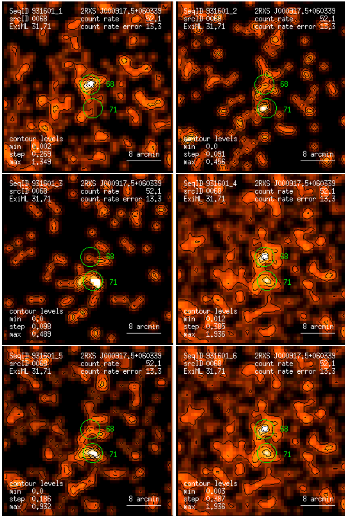
Figure 68: RASS 931601: detection 0068: band rate images, Gaussian filter: (1) PSPC channels 11 – 41, (2) 52 – 90, (3) 91 – 201, (4) 11 – 235, (5) 52 – 201, (6) 11 – 201. Broad band rates in counts/ks. Band rate contour levels in counts/ks/arcmin 2 .
