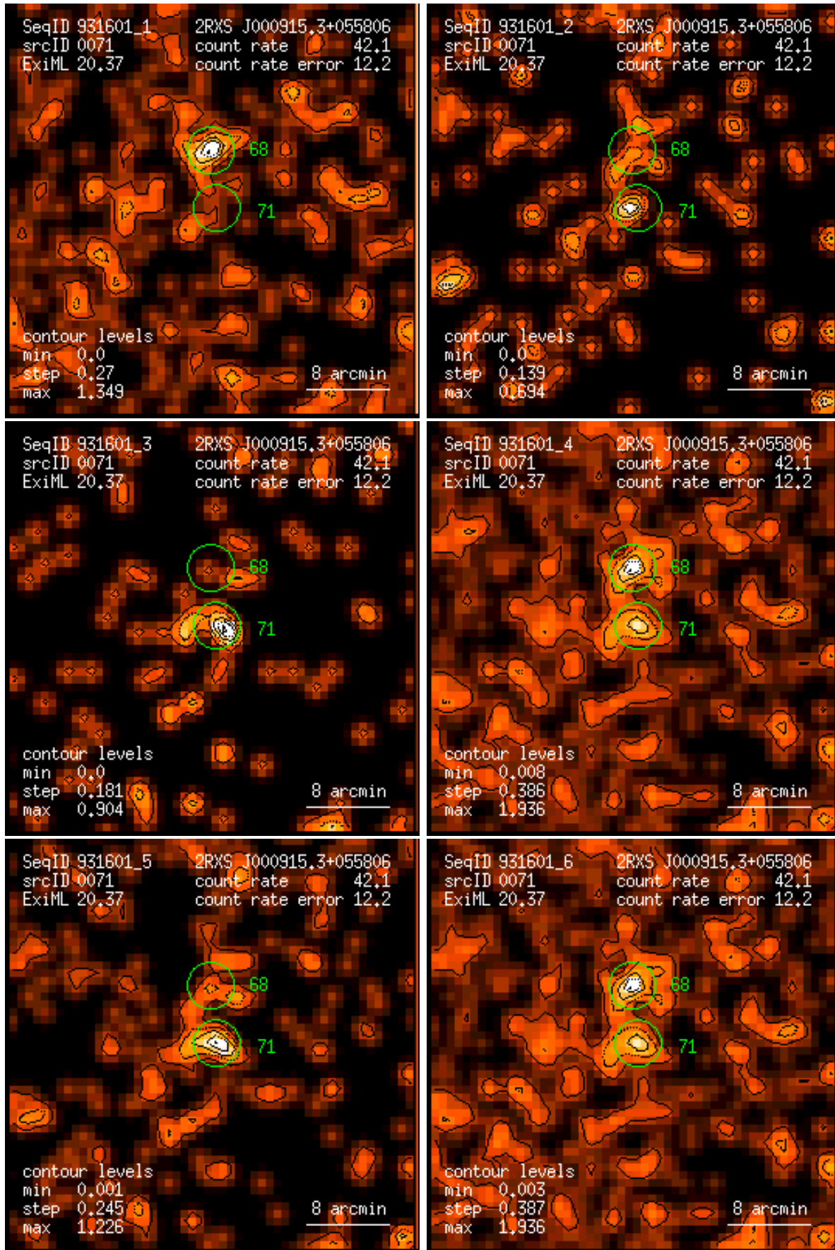
Figure 71: RASS 931601: detection 0071: band rate images, Gaussian filter: (1) PSPC channels 11 – 41, (2) 52 – 90, (3) 91 – 201, (4) 11 – 235, (5) 52 – 201, (6) 11 – 201. Broad band rates in counts/ks. Band rate contour levels in counts/ks/arcmin 2 .
