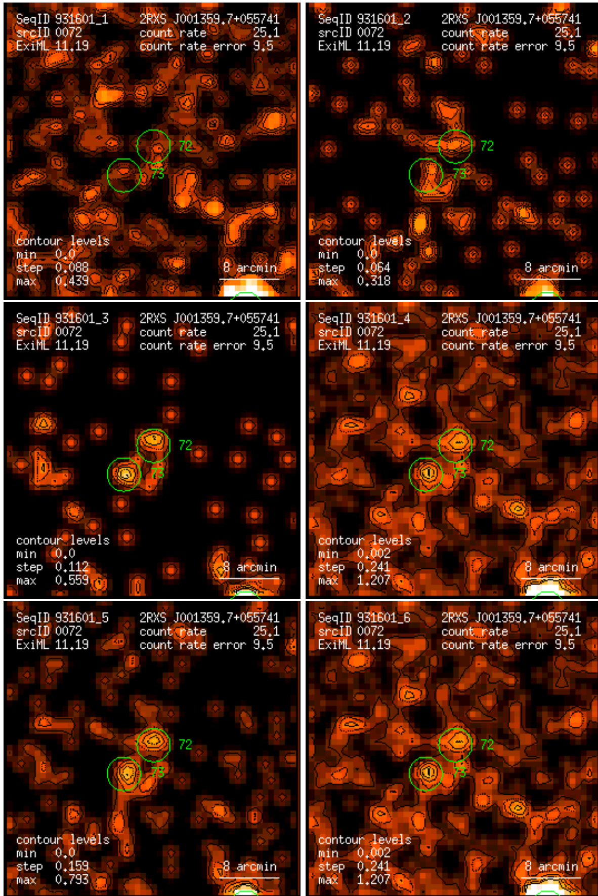
Figure 72: RASS 931601: detection 0072: band rate images, Gaussian filter: (1) PSPC channels 11 – 41, (2) 52 – 90, (3) 91 – 201, (4) 11 – 235, (5) 52 – 201, (6) 11 – 201. Broad band rates in counts/ks. Band rate contour levels in counts/ks/arcmin 2 .
