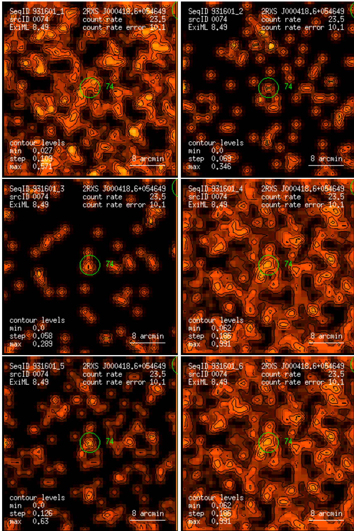
Figure 74: RASS 931601: detection 0074: band rate images, Gaussian filter: (1) PSPC channels 11 – 41, (2) 52 – 90, (3) 91 – 201, (4) 11 – 235, (5) 52 – 201, (6) 11 – 201. Broad band rates in counts/ks. Band rate contour levels in counts/ks/arcmin 2 .
