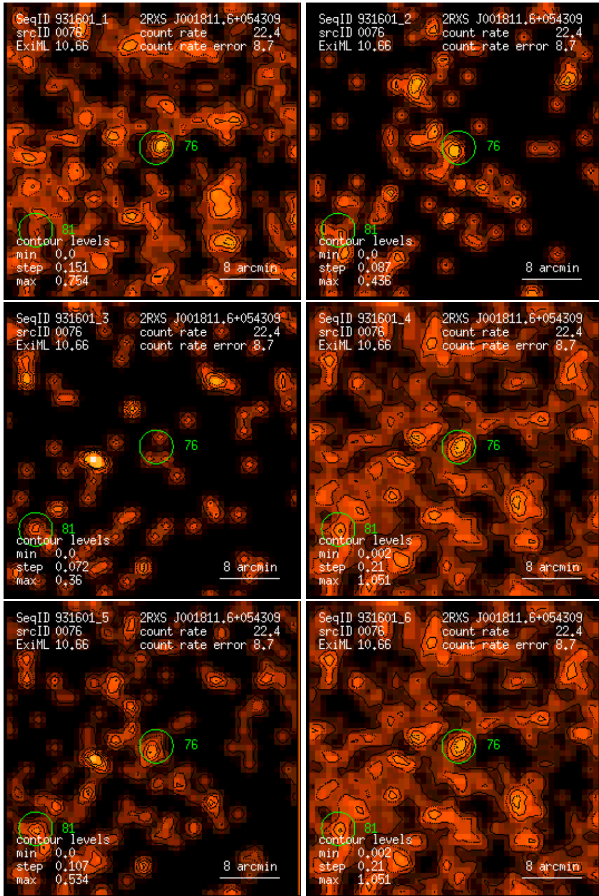
Figure 76: RASS 931601: detection 0076: band rate images, Gaussian filter: (1) PSPC channels 11 – 41, (2) 52 – 90, (3) 91 – 201, (4) 11 – 235, (5) 52 – 201, (6) 11 – 201. Broad band rates in counts/ks. Band rate contour levels in counts/ks/arcmin 2 .
