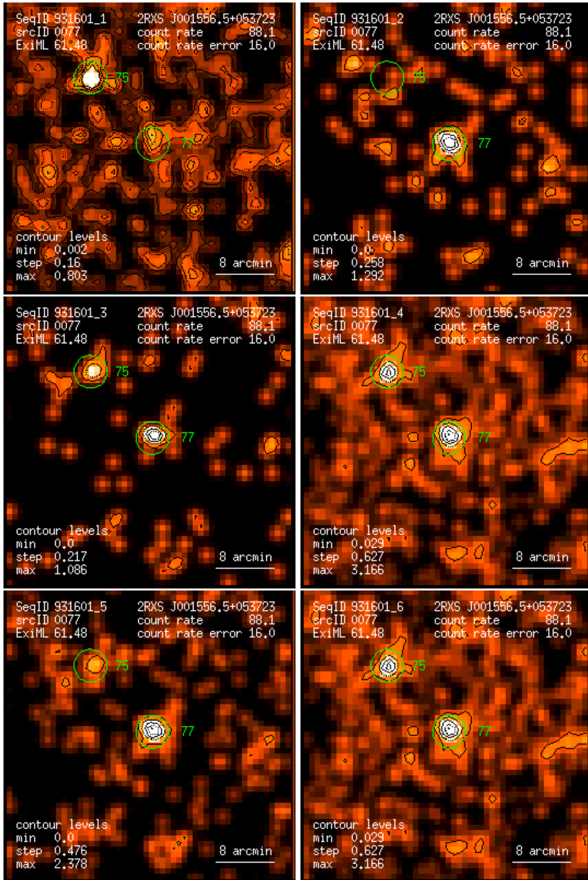
Figure 77: RASS 931601: detection 0077: band rate images, Gaussian filter: (1) PSPC channels 11 – 41, (2) 52 – 90, (3) 91 – 201, (4) 11 – 235, (5) 52 – 201, (6) 11 – 201. Broad band rates in counts/ks. Band rate contour levels in counts/ks/arcmin 2 .
