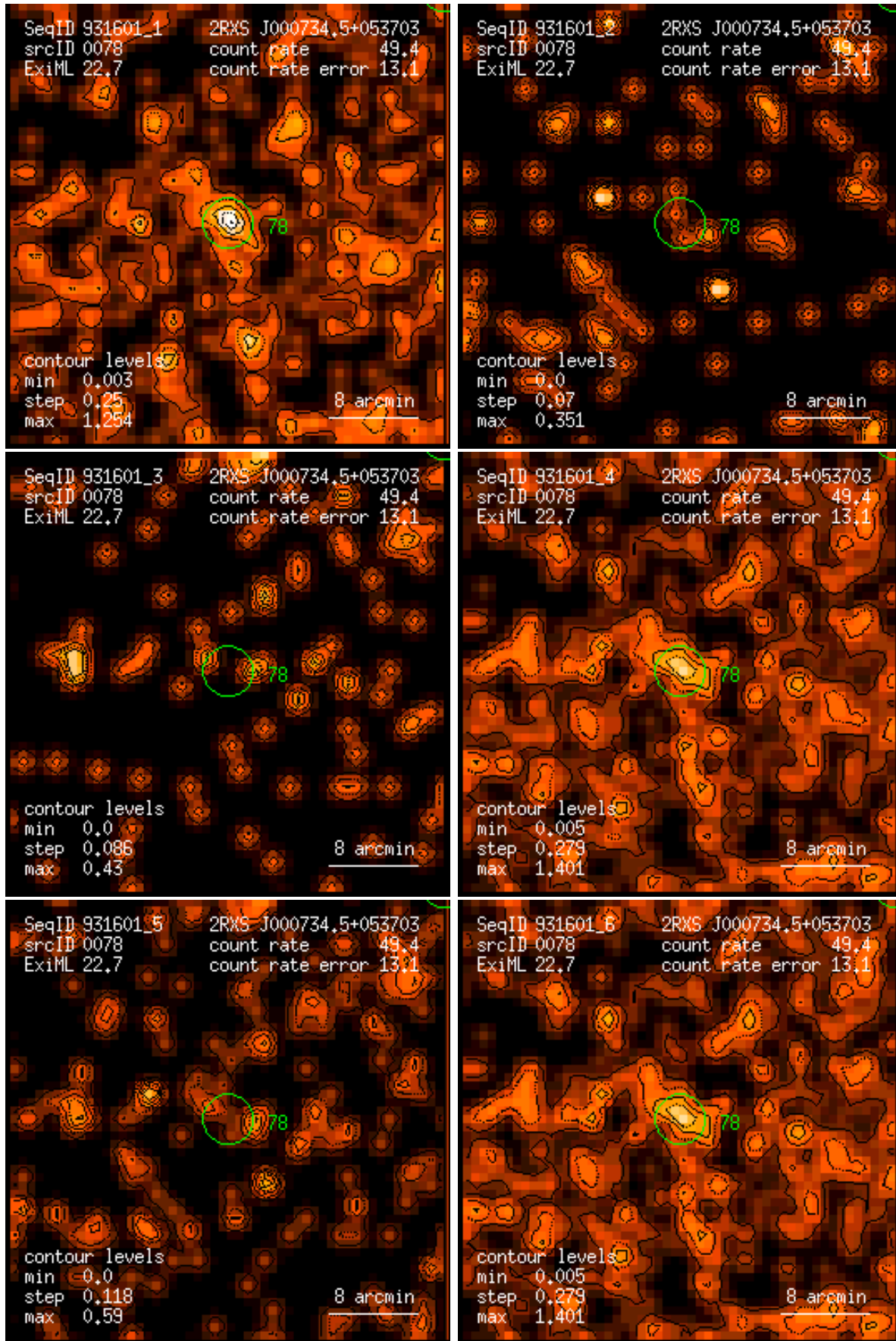
Figure 78: RASS 931601: detection 0078: band rate images, Gaussian filter: (1) PSPC channels 11 – 41, (2) 52 – 90, (3) 91 – 201, (4) 11 – 235, (5) 52 – 201, (6) 11 – 201. Broad band rates in counts/ks. Band rate contour levels in counts/ks/arcmin 2 .
