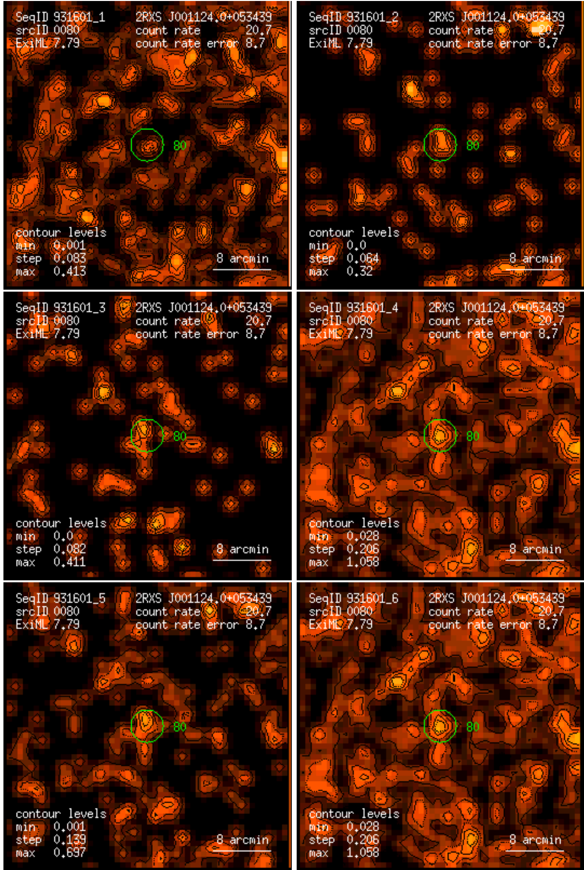
Figure 80: RASS 931601: detection 0080: band rate images, Gaussian filter: (1) PSPC channels 11 – 41, (2) 52 – 90, (3) 91 – 201, (4) 11 – 235, (5) 52 – 201, (6) 11 – 201. Broad band rates in counts/ks. Band rate contour levels in counts/ks/arcmin 2 .
