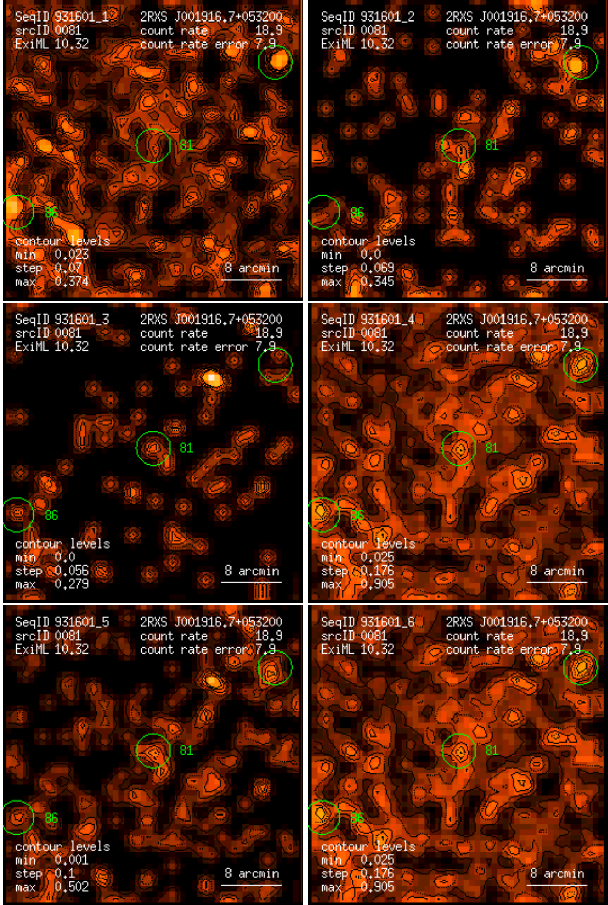
Figure 81: RASS 931601: detection 0081: band rate images, Gaussian filter: (1) PSPC channels 11 – 41, (2) 52 – 90, (3) 91 – 201, (4) 11 – 235, (5) 52 – 201, (6) 11 – 201. Broad band rates in counts/ks. Band rate contour levels in counts/ks/arcmin 2 .
