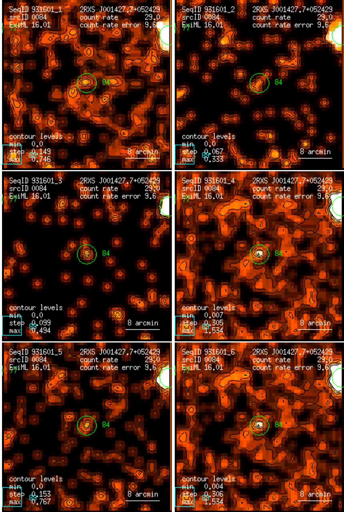
Figure 84: RASS 931601: detection 0084: band rate images, Gaussian filter: (1) PSPC channels 11 – 41, (2) 52 – 90, (3) 91 – 201, (4) 11 – 235, (5) 52 – 201, (6) 11 – 201. Broad band rates in counts/ks. Band rate contour levels in counts/ks/arcmin 2 .
