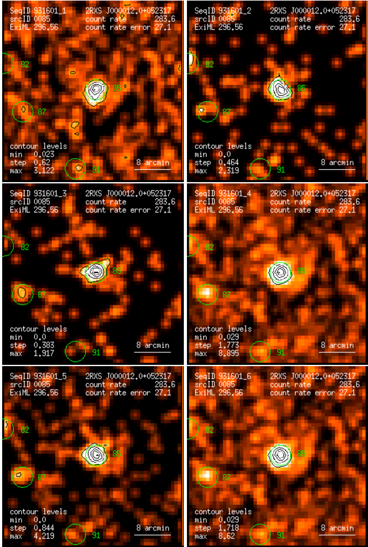
Figure 85: RASS 931601: detection 0085: band rate images, Gaussian filter: (1) PSPC channels 11 – 41, (2) 52 – 90, (3) 91 – 201, (4) 11 – 235, (5) 52 – 201, (6) 11 – 201. Broad band rates in counts/ks. Band rate contour levels in counts/ks/arcmin 2 .
