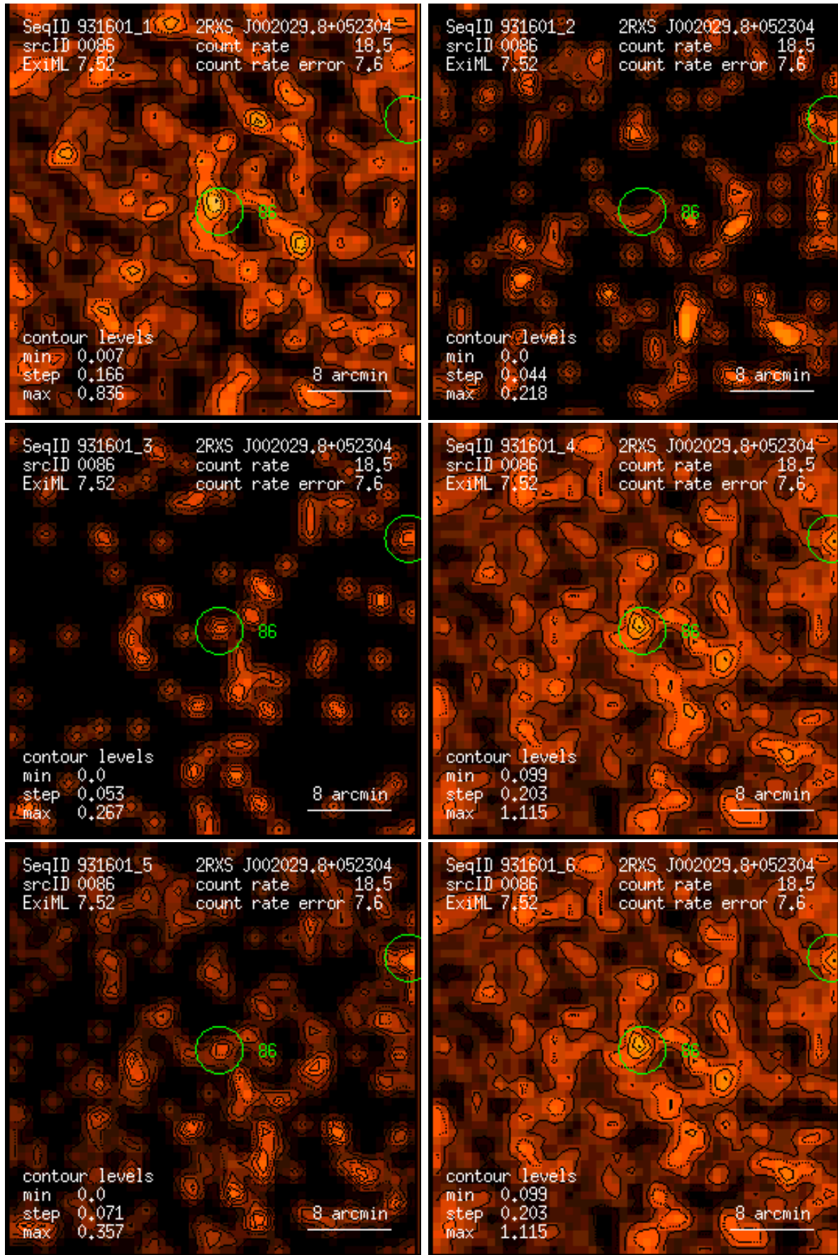
Figure 86: RASS 931601: detection 0086: band rate images, Gaussian filter: (1) PSPC channels 11 – 41, (2) 52 – 90, (3) 91 – 201, (4) 11 – 235, (5) 52 – 201, (6) 11 – 201. Broad band rates in counts/ks. Band rate contour levels in counts/ks/arcmin 2 .
