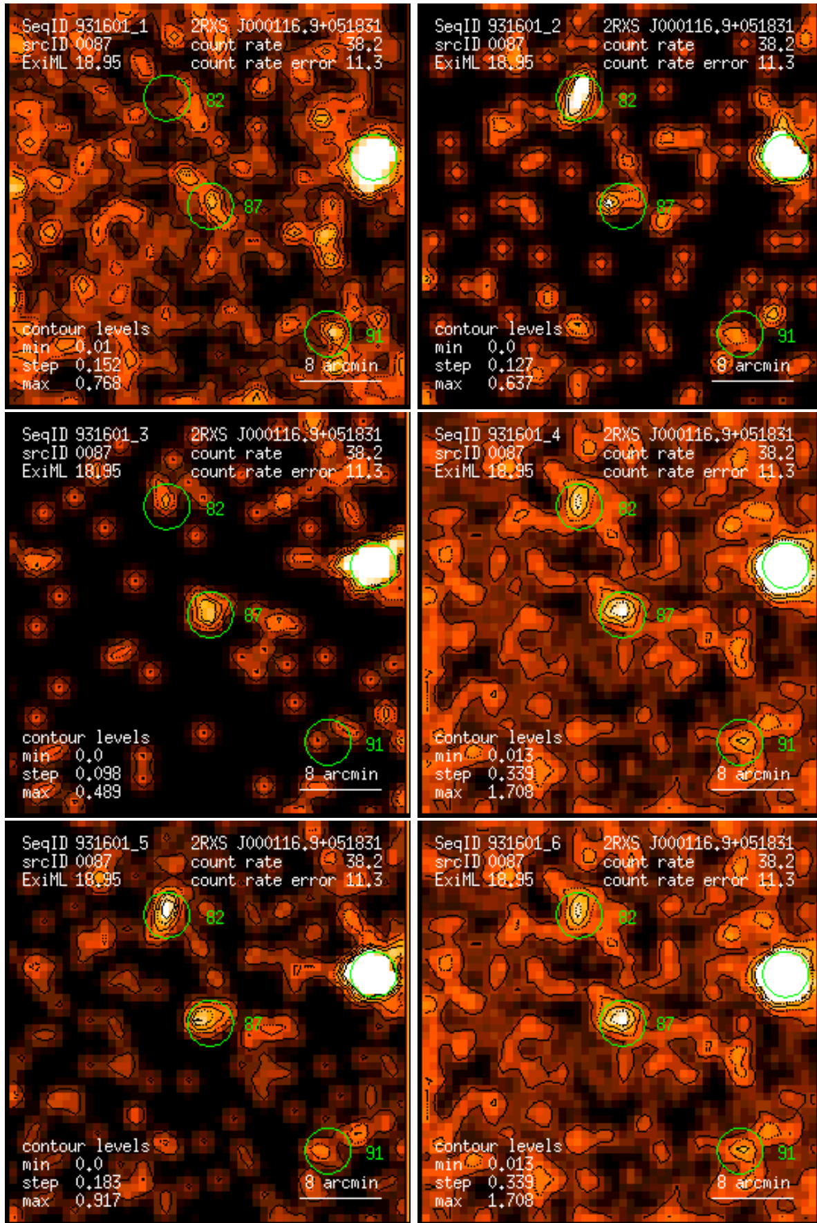
Figure 87: RASS 931601: detection 0087: band rate images, Gaussian filter: (1) PSPC channels 11 – 41, (2) 52 – 90, (3) 91 – 201, (4) 11 – 235, (5) 52 – 201, (6) 11 – 201. Broad band rates in counts/ks. Band rate contour levels in counts/ks/arcmin 2 .
