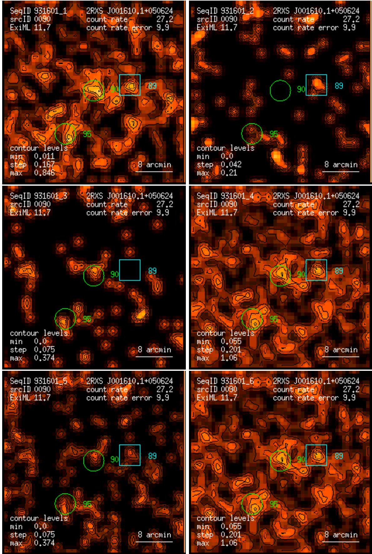
Figure 90: RASS 931601: detection 0090: band rate images, Gaussian filter: (1) PSPC channels 11 – 41, (2) 52 – 90, (3) 91 – 201, (4) 11 – 235, (5) 52 – 201, (6) 11 – 201. Broad band rates in counts/ks. Band rate contour levels in counts/ks/arcmin 2 .
