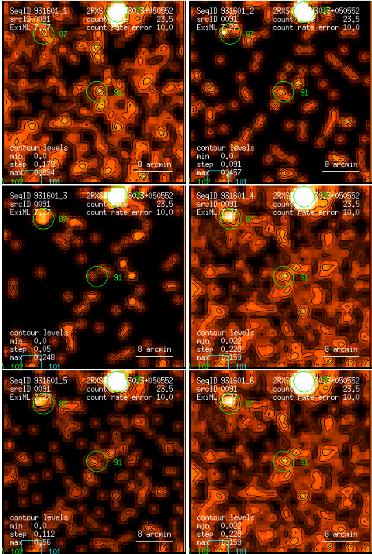
Figure 91: RASS 931601: detection 0091: band rate images, Gaussian filter: (1) PSPC channels 11 – 41, (2) 52 – 90, (3) 91 – 201, (4) 11 – 235, (5) 52 – 201, (6) 11 – 201. Broad band rates in counts/ks. Band rate contour levels in counts/ks/arcmin 2 .
