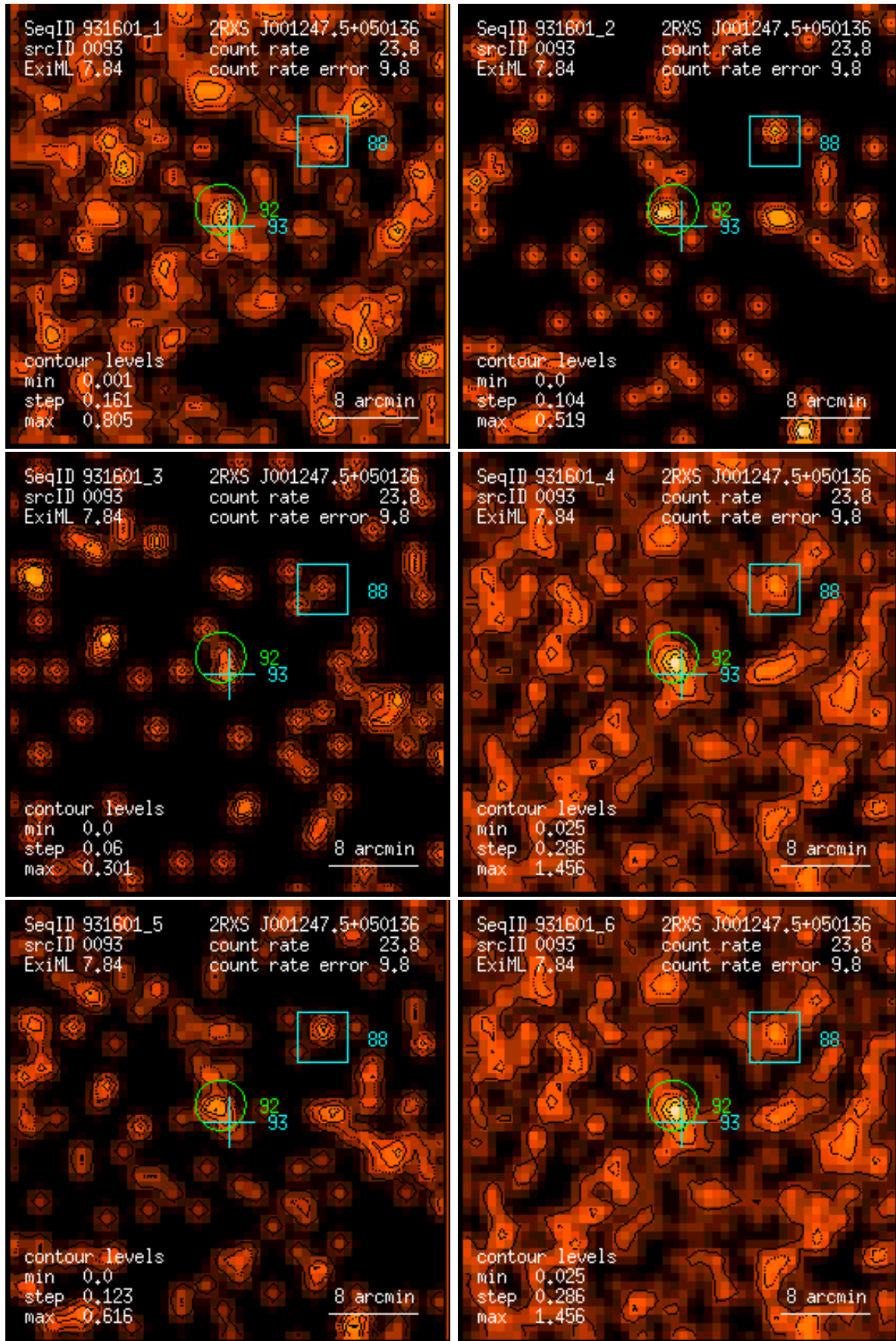
Figure 93: RASS 931601: detection 0093: band rate images, Gaussian filter: (1) PSPC channels 11 – 41, (2) 52 – 90, (3) 91 – 201, (4) 11 – 235, (5) 52 – 201, (6) 11 – 201. Broad band rates in counts/ks. Band rate contour levels in counts/ks/arcmin 2 .
