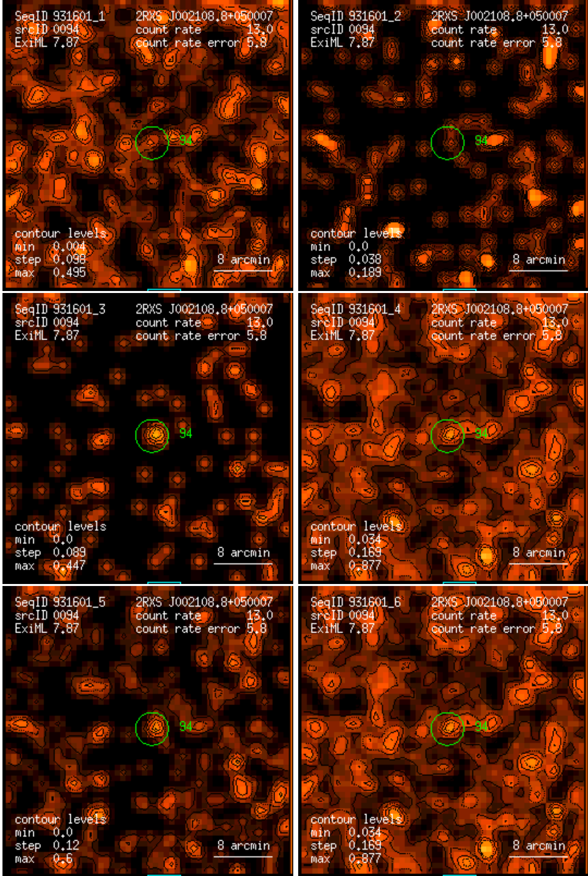
Figure 94: RASS 931601: detection 0094: band rate images, Gaussian filter: (1) PSPC channels 11 – 41, (2) 52 – 90, (3) 91 – 201, (4) 11 – 235, (5) 52 – 201, (6) 11 – 201. Broad band rates in counts/ks. Band rate contour levels in counts/ks/arcmin 2 .
