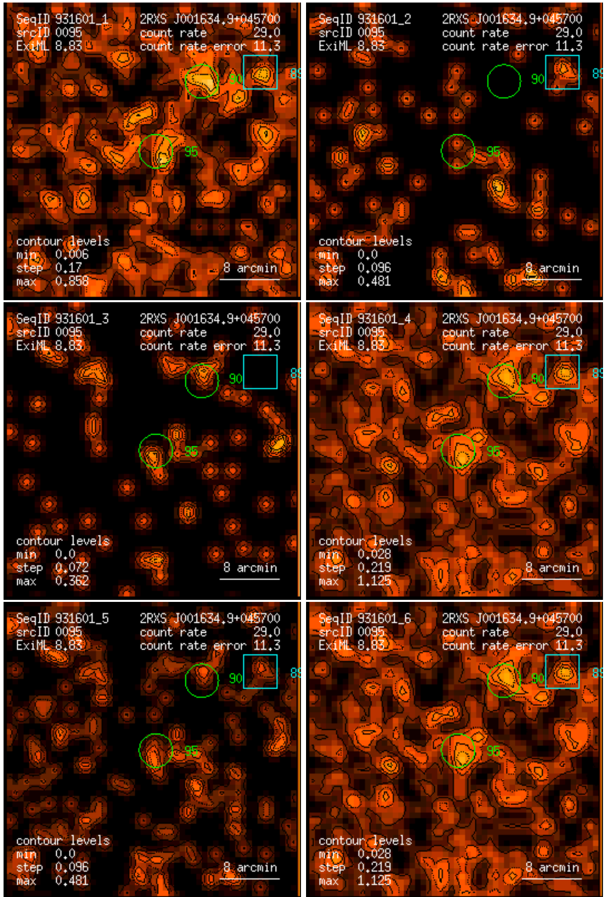
Figure 95: RASS 931601: detection 0095: band rate images, Gaussian filter: (1) PSPC channels 11 – 41, (2) 52 – 90, (3) 91 – 201, (4) 11 – 235, (5) 52 – 201, (6) 11 – 201. Broad band rates in counts/ks. Band rate contour levels in counts/ks/arcmin 2 .
