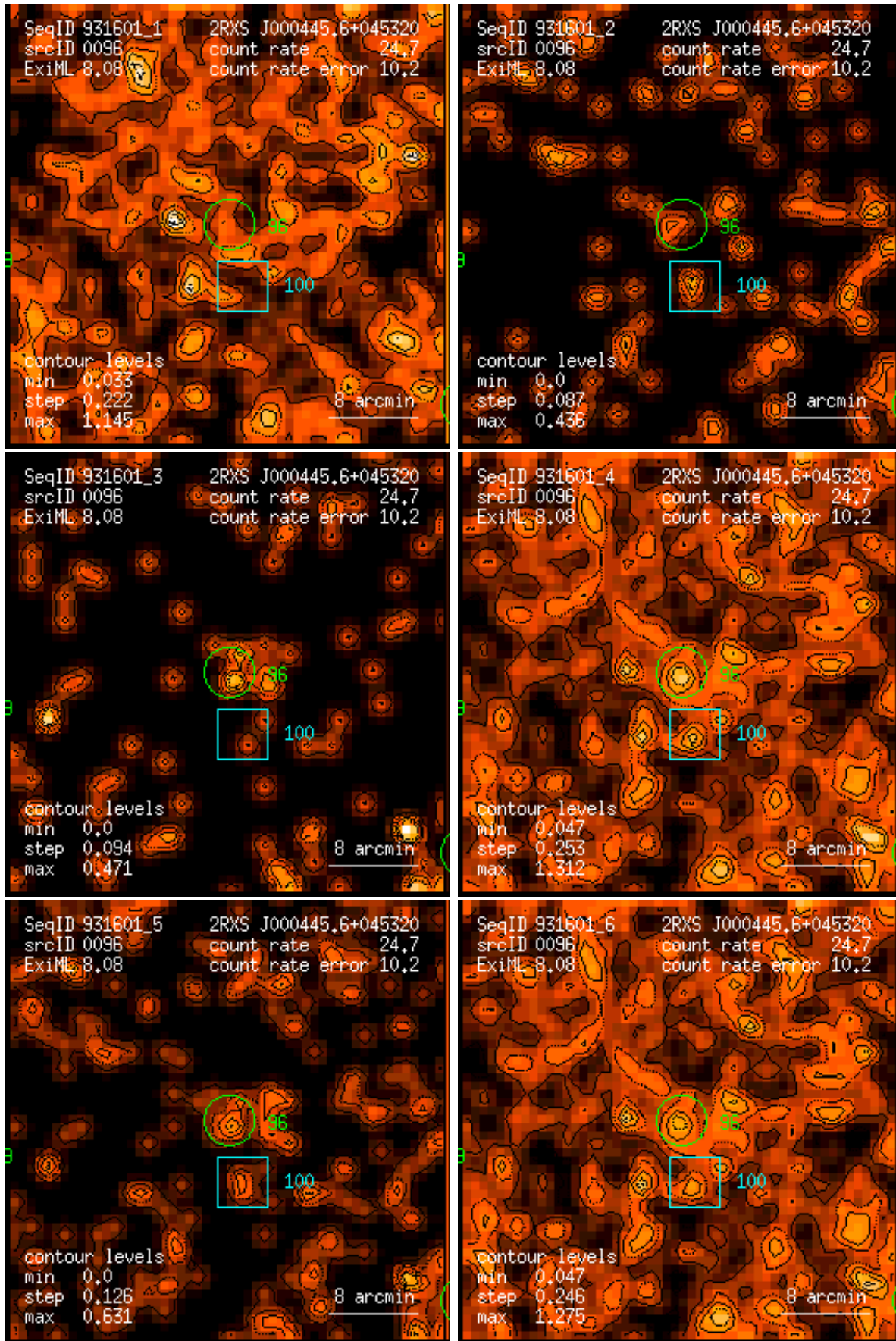
Figure 96: RASS 931601: detection 0096: band rate images, Gaussian filter: (1) PSPC channels 11 – 41, (2) 52 – 90, (3) 91 – 201, (4) 11 – 235, (5) 52 – 201, (6) 11 – 201. Broad band rates in counts/ks. Band rate contour levels in counts/ks/arcmin 2 .
