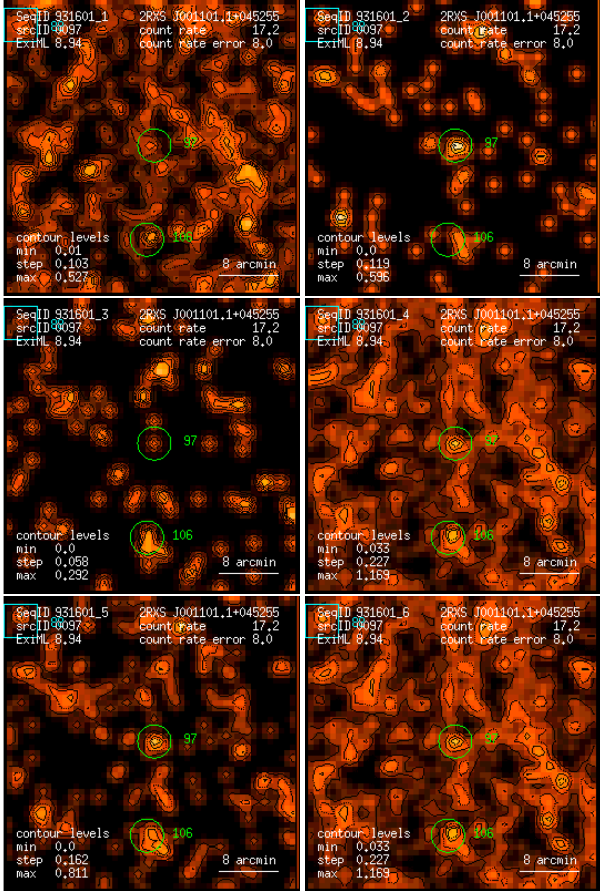
Figure 97: RASS 931601: detection 0097: band rate images, Gaussian filter: (1) PSPC channels 11 – 41, (2) 52 – 90, (3) 91 – 201, (4) 11 – 235, (5) 52 – 201, (6) 11 – 201. Broad band rates in counts/ks. Band rate contour levels in counts/ks/arcmin 2 .
