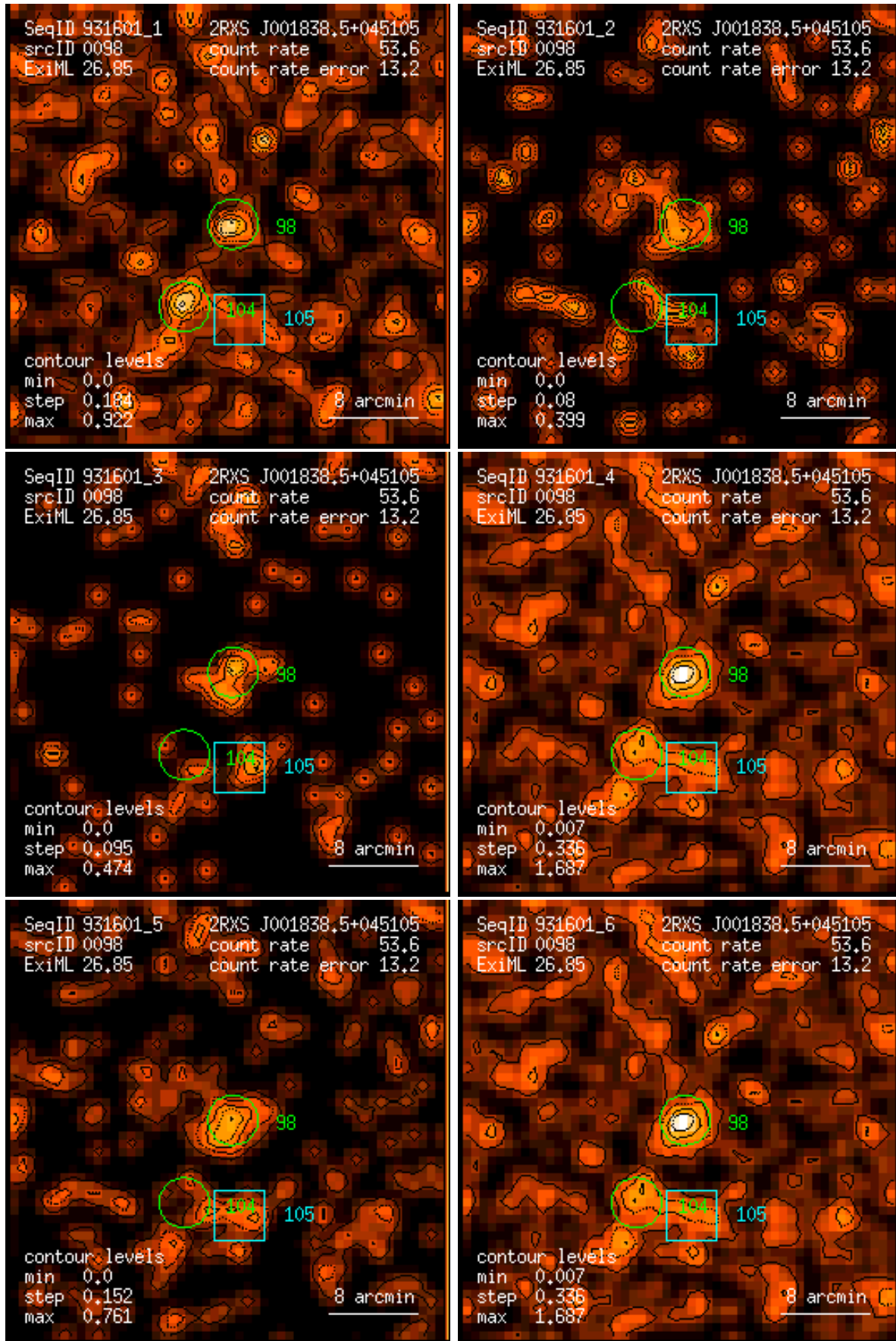
Figure 98: RASS 931601: detection 0098: band rate images, Gaussian filter: (1) PSPC channels 11 – 41, (2) 52 – 90, (3) 91 – 201, (4) 11 – 235, (5) 52 – 201, (6) 11 – 201. Broad band rates in counts/ks. Band rate contour levels in counts/ks/arcmin 2 .
