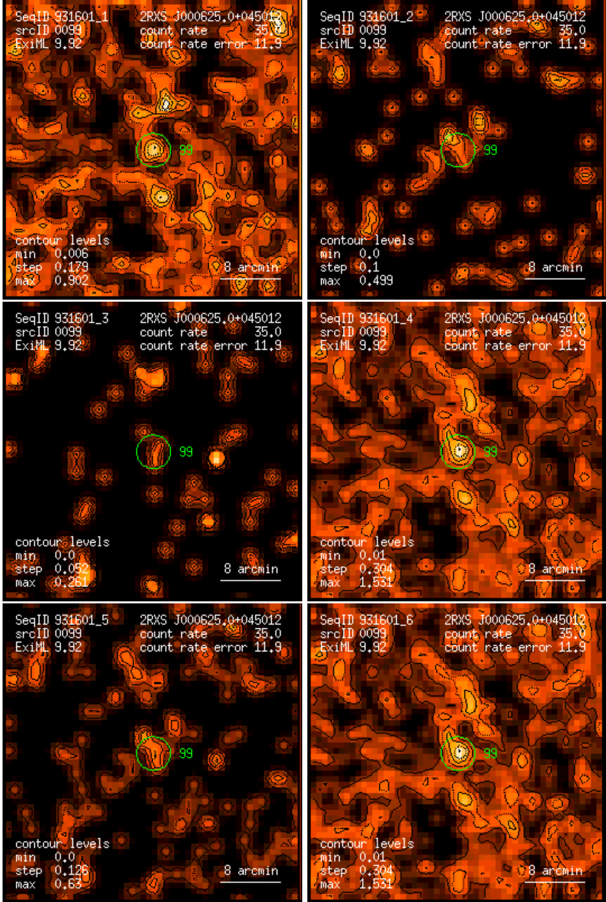
Figure 99: RASS 931601: detection 0099: band rate images, Gaussian filter: (1) PSPC channels 11 – 41, (2) 52 – 90, (3) 91 – 201, (4) 11 – 235, (5) 52 – 201, (6) 11 – 201. Broad band rates in counts/ks. Band rate contour levels in counts/ks/arcmin 2 .
