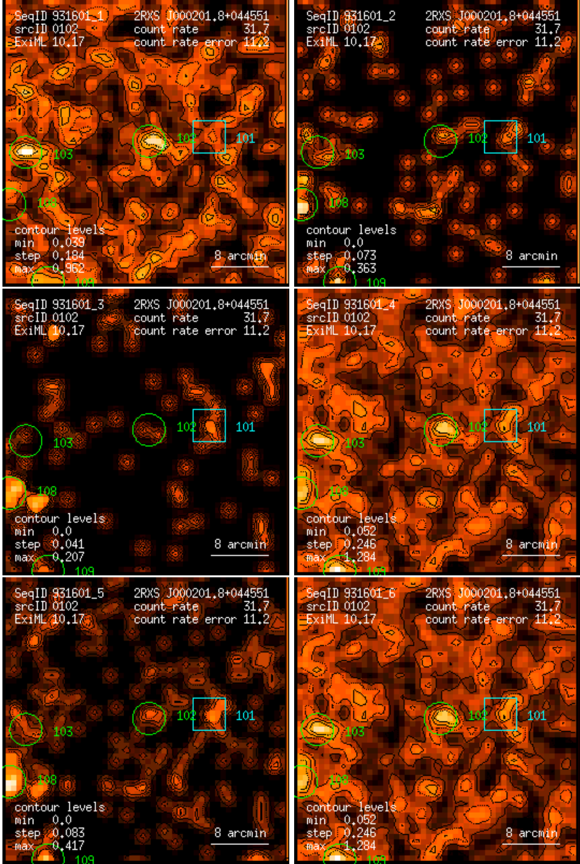
Figure 102: RASS 931601: detection 0102: band rate images, Gaussian filter: (1) PSPC channels 11 – 41, (2) 52 – 90, (3) 91 – 201, (4) 11 – 235, (5) 52 – 201, (6) 11 – 201. Broad band rates in counts/ks. Band rate contour levels in counts/ks/arcmin 2 .
