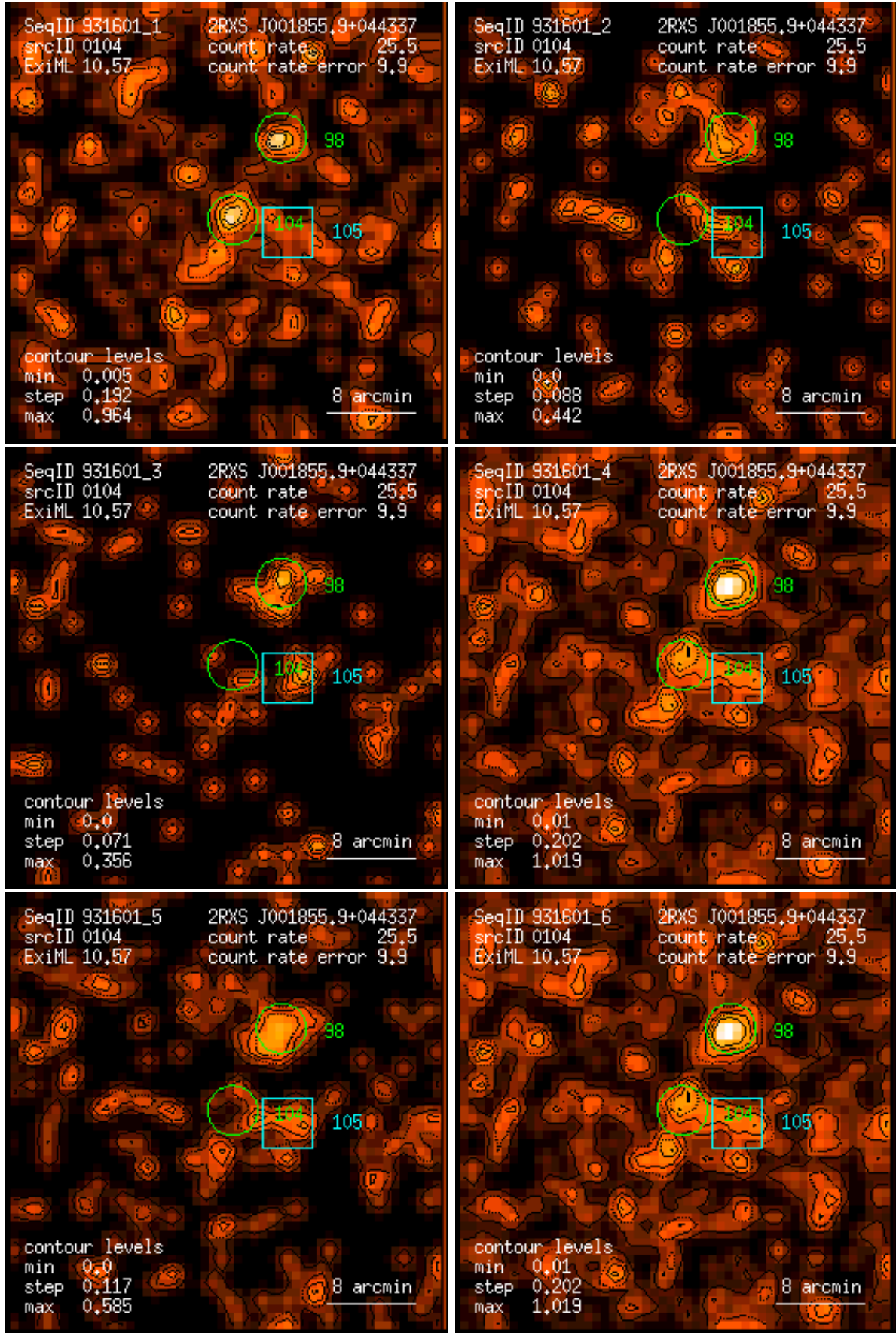
Figure 104: RASS 931601: detection 0104: band rate images, Gaussian filter: (1) PSPC channels 11 – 41, (2) 52 – 90, (3) 91 – 201, (4) 11 – 235, (5) 52 – 201, (6) 11 – 201. Broad band rates in counts/ks. Band rate contour levels in counts/ks/arcmin 2 .
