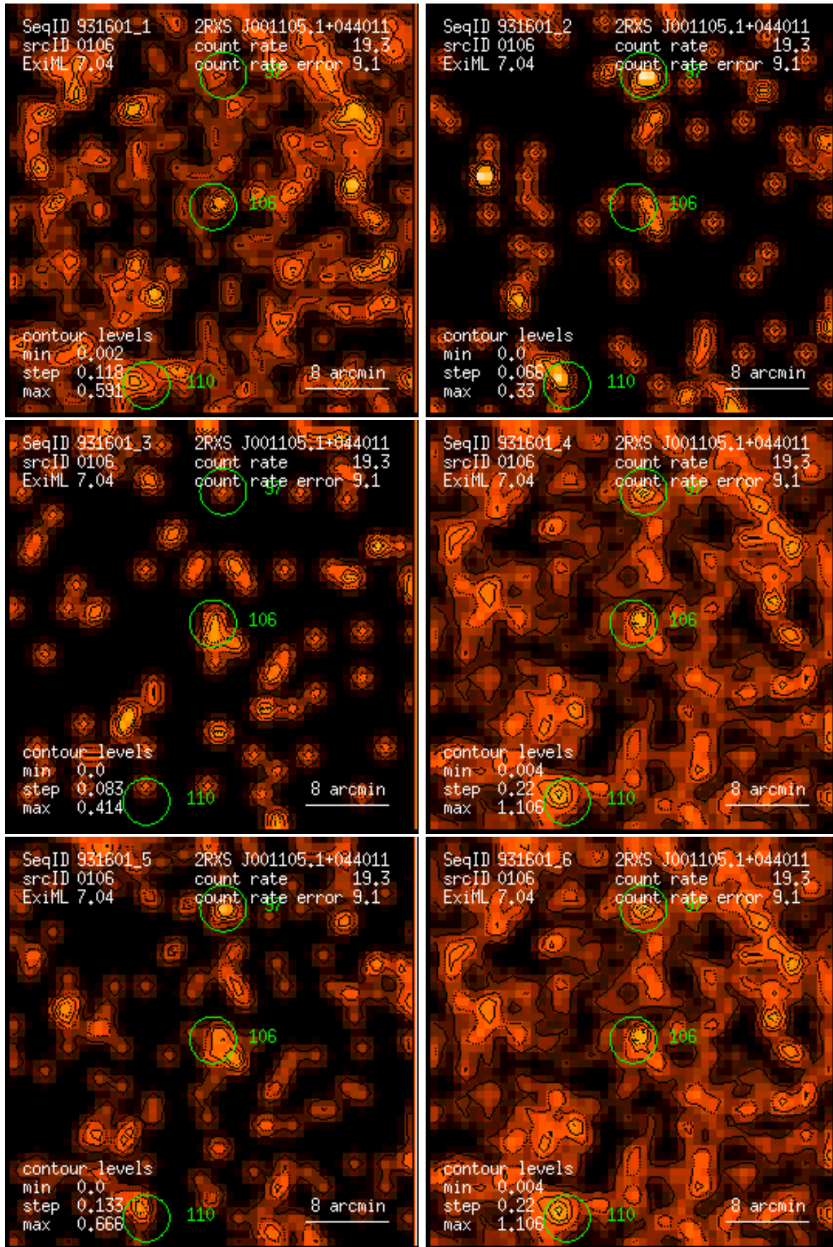
Figure 106: RASS 931601: detection 0106: band rate images, Gaussian filter: (1) PSPC channels 11 – 41, (2) 52 – 90, (3) 91 – 201, (4) 11 – 235, (5) 52 – 201, (6) 11 – 201. Broad band rates in counts/ks. Band rate contour levels in counts/ks/arcmin 2 .
