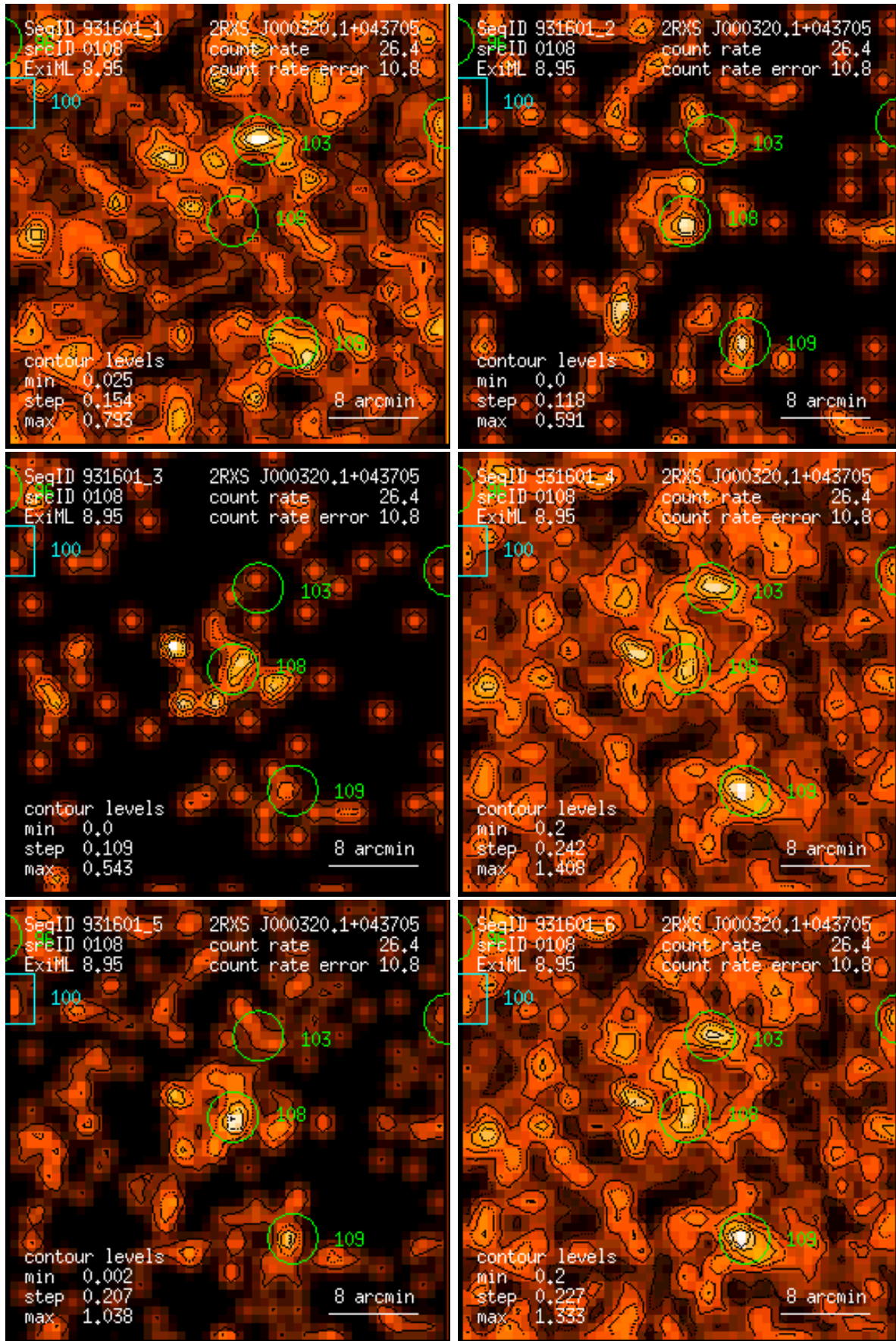
Figure 108: RASS 931601: detection 0108: band rate images, Gaussian filter: (1) PSPC channels 11 – 41, (2) 52 – 90, (3) 91 – 201, (4) 11 – 235, (5) 52 – 201, (6) 11 – 201. Broad band rates in counts/ks. Band rate contour levels in counts/ks/arcmin 2 .
