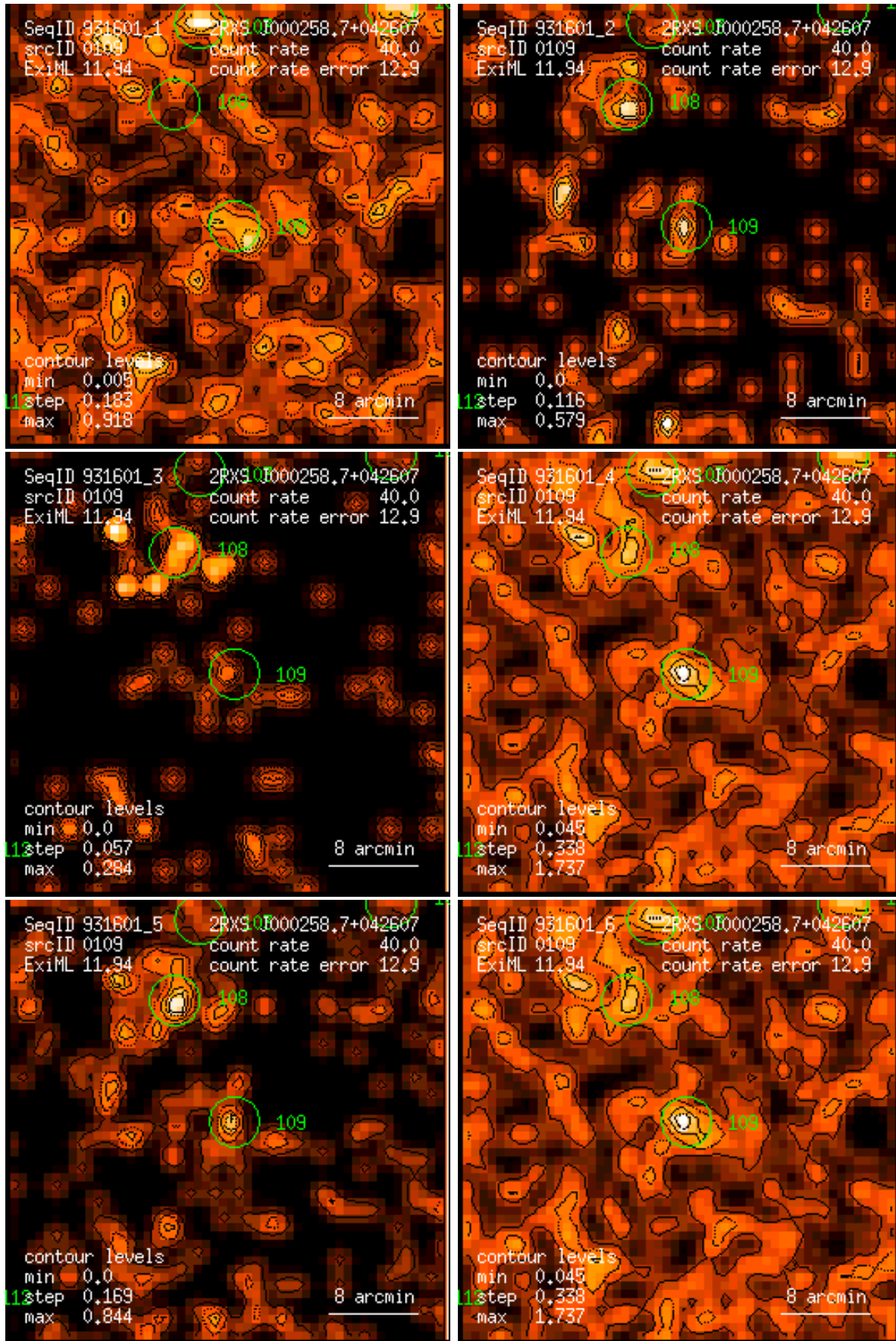
Figure 109: RASS 931601: detection 0109: band rate images, Gaussian filter: (1) PSPC channels 11 – 41, (2) 52 – 90, (3) 91 – 201, (4) 11 – 235, (5) 52 – 201, (6) 11 – 201. Broad band rates in counts/ks. Band rate contour levels in counts/ks/arcmin 2 .
