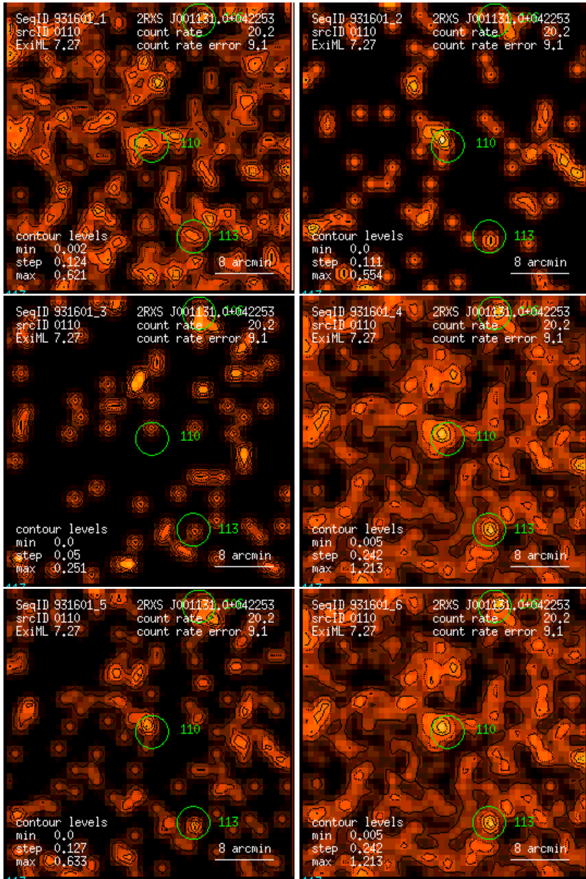
Figure 110: RASS 931601: detection 0110: band rate images, Gaussian filter: (1) PSPC channels 11 – 41, (2) 52 – 90, (3) 91 – 201, (4) 11 – 235, (5) 52 – 201, (6) 11 – 201. Broad band rates in counts/ks. Band rate contour levels in counts/ks/arcmin 2 .
