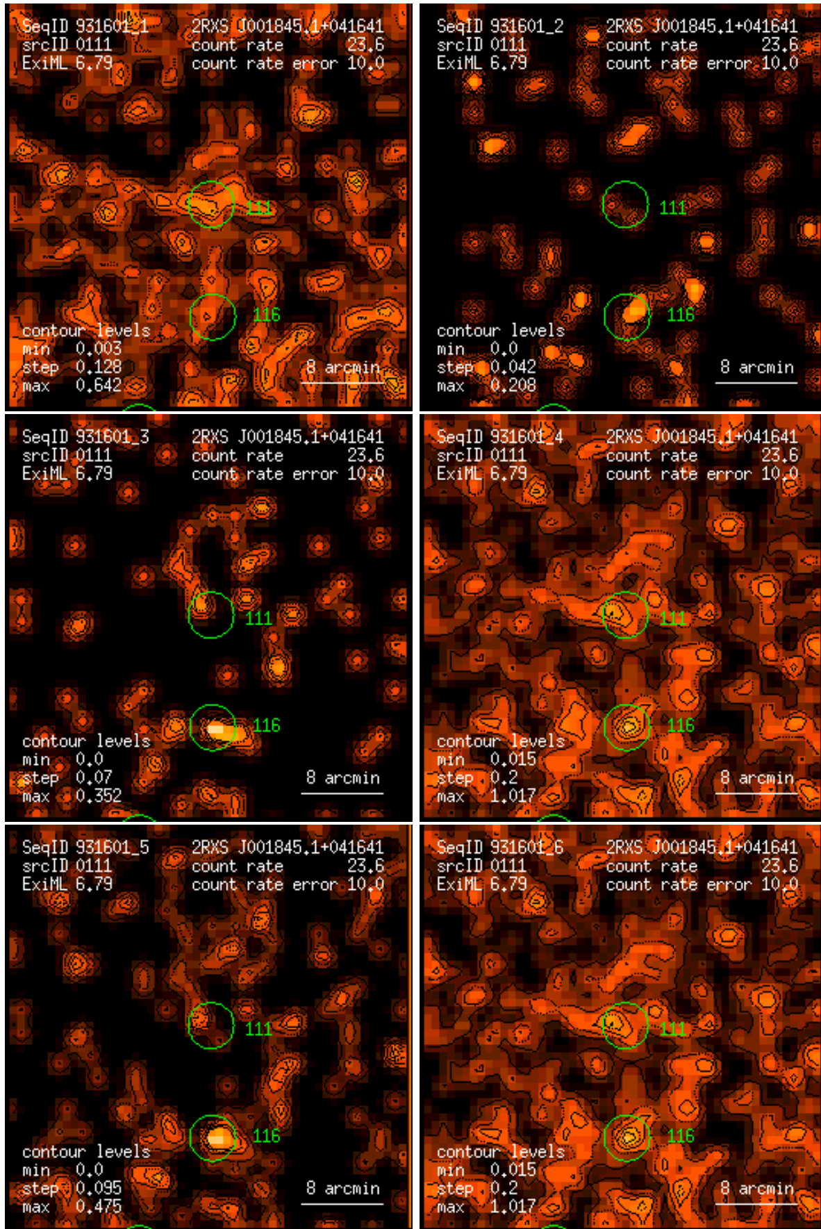
Figure 111: RASS 931601: detection 0111: band rate images, Gaussian filter: (1) PSPC channels 11 – 41, (2) 52 – 90, (3) 91 – 201, (4) 11 – 235, (5) 52 – 201, (6) 11 – 201. Broad band rates in counts/ks. Band rate contour levels in counts/ks/arcmin 2 .
