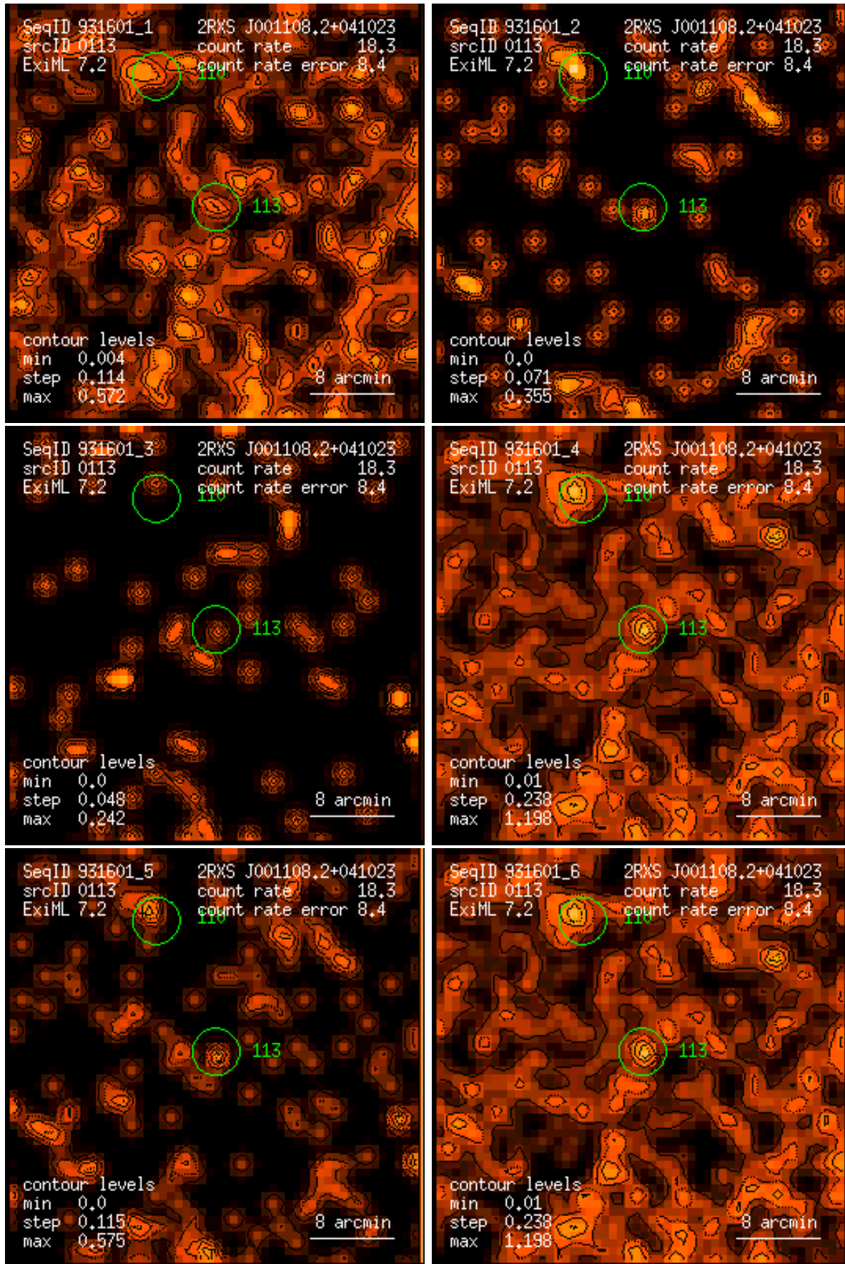
Figure 113: RASS 931601: detection 0113: band rate images, Gaussian filter: (1) PSPC channels 11 – 41, (2) 52 – 90, (3) 91 – 201, (4) 11 – 235, (5) 52 – 201, (6) 11 – 201. Broad band rates in counts/ks. Band rate contour levels in counts/ks/arcmin 2 .
