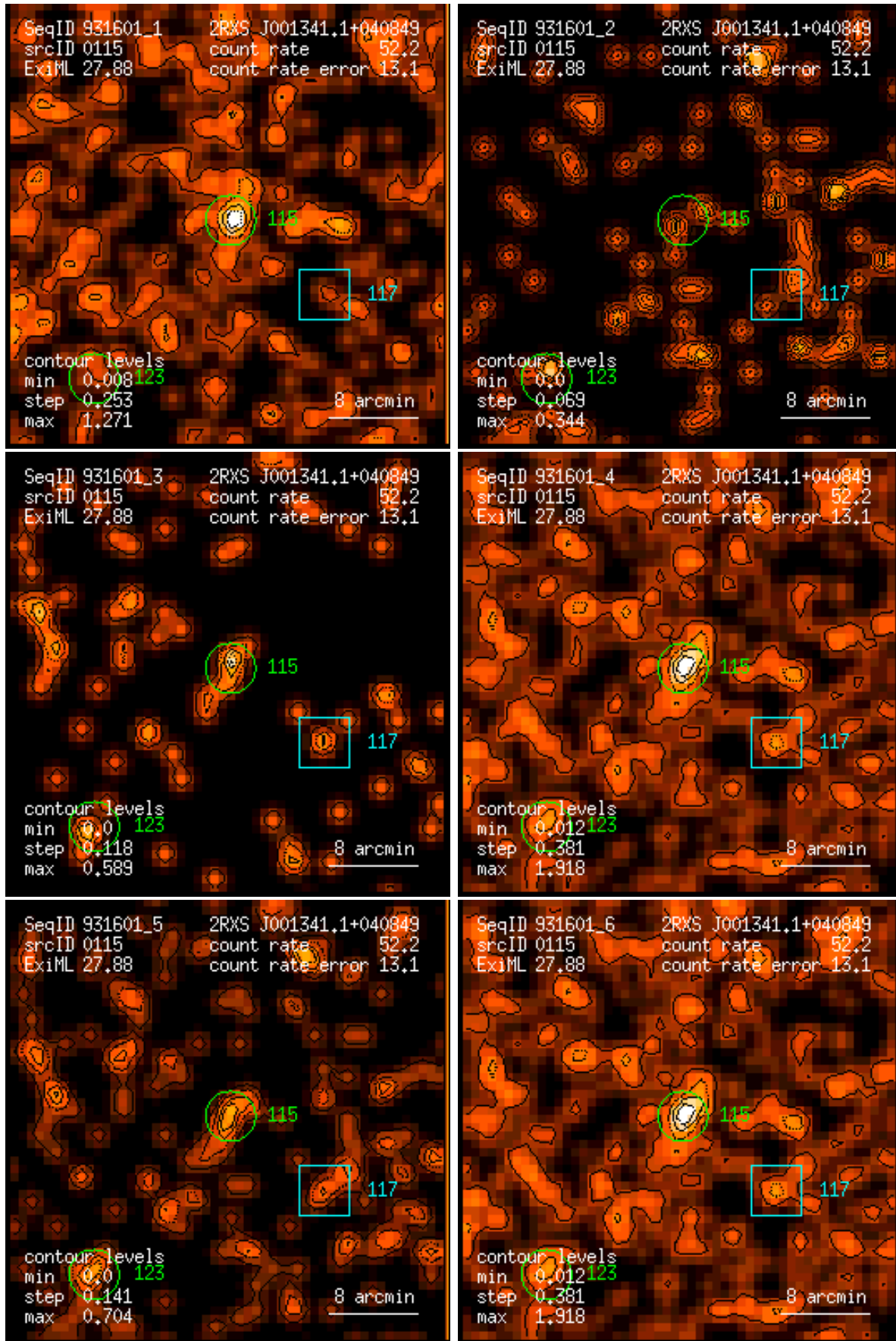
Figure 115: RASS 931601: detection 0115: band rate images, Gaussian filter: (1) PSPC channels 11 – 41, (2) 52 – 90, (3) 91 – 201, (4) 11 – 235, (5) 52 – 201, (6) 11 – 201. Broad band rates in counts/ks. Band rate contour levels in counts/ks/arcmin 2 .
