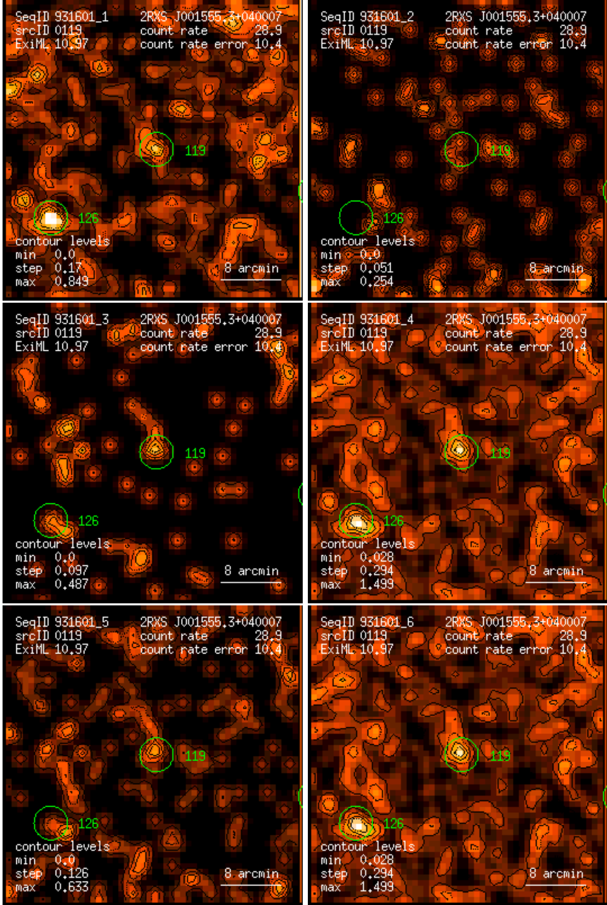
Figure 119: RASS 931601: detection 0119: band rate images, Gaussian filter: (1) PSPC channels 11 – 41, (2) 52 – 90, (3) 91 – 201, (4) 11 – 235, (5) 52 – 201, (6) 11 – 201. Broad band rates in counts/ks. Band rate contour levels in counts/ks/arcmin 2 .
