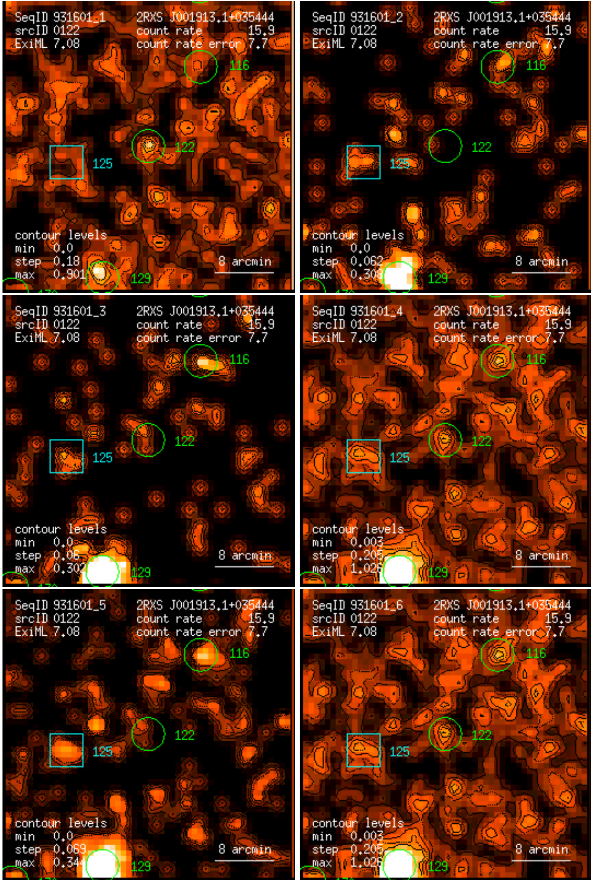
Figure 122: RASS 931601: detection 0122: band rate images, Gaussian filter: (1) PSPC channels 11 – 41, (2) 52 – 90, (3) 91 – 201, (4) 11 – 235, (5) 52 – 201, (6) 11 – 201. Broad band rates in counts/ks. Band rate contour levels in counts/ks/arcmin 2 .
