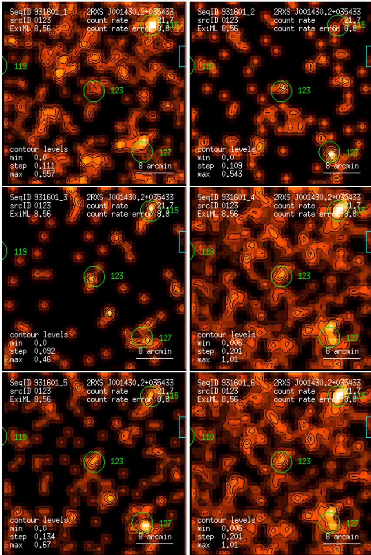
Figure 123: RASS 931601: detection 0123: band rate images, Gaussian filter: (1) PSPC channels 11 – 41, (2) 52 – 90, (3) 91 – 201, (4) 11 – 235, (5) 52 – 201, (6) 11 – 201. Broad band rates in counts/ks. Band rate contour levels in counts/ks/arcmin 2 .
