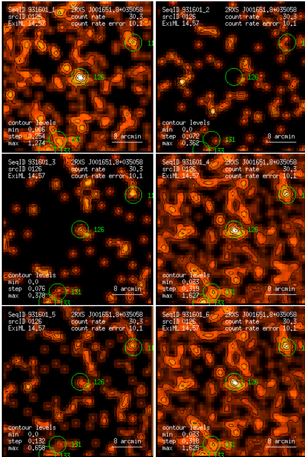
Figure 126: RASS 931601: detection 0126: band rate images, Gaussian filter: (1) PSPC channels 11 – 41, (2) 52 – 90, (3) 91 – 201, (4) 11 – 235, (5) 52 – 201, (6) 11 – 201. Broad band rates in counts/ks. Band rate contour levels in counts/ks/arcmin 2 .
