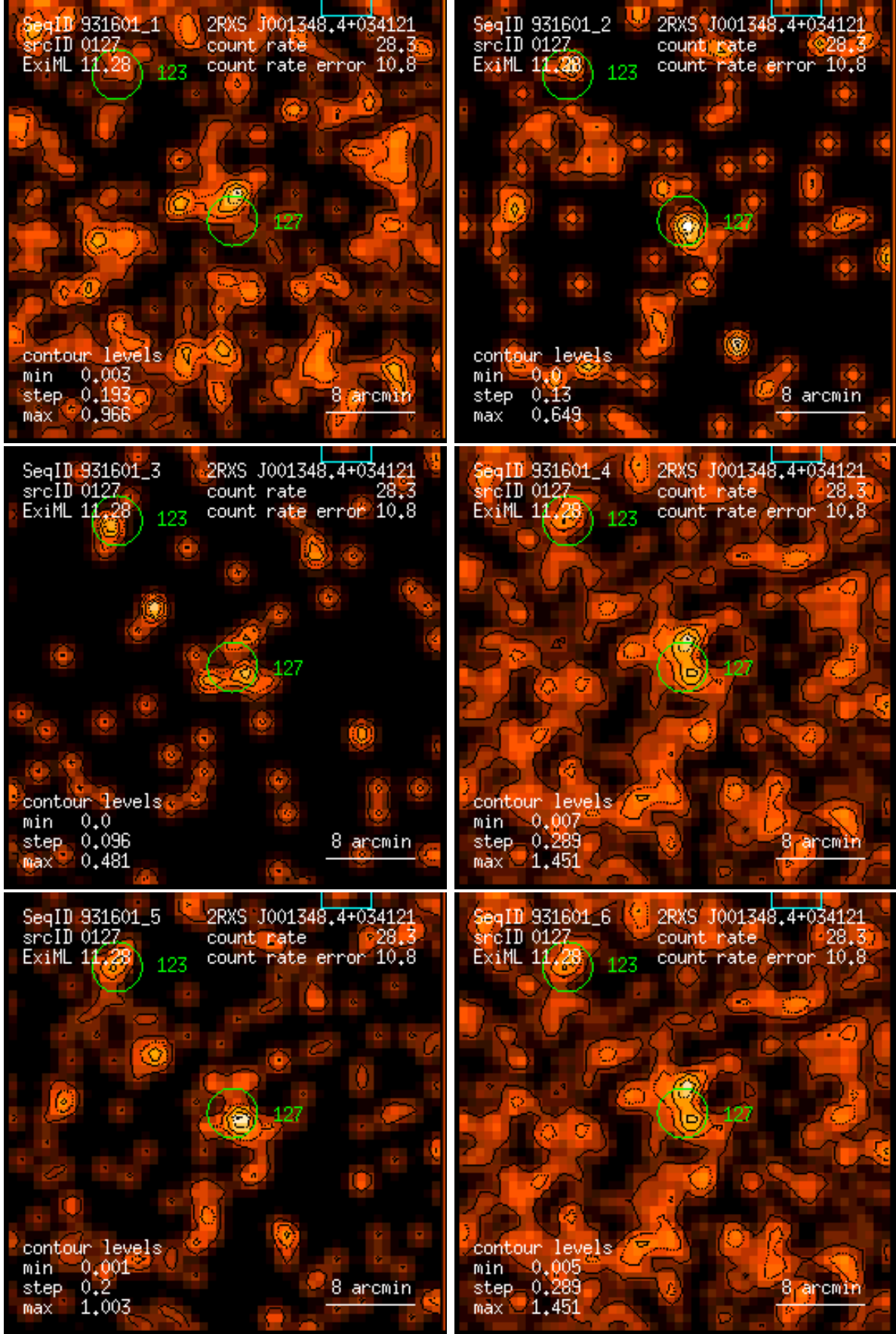
Figure 127: RASS 931601: detection 0127: band rate images, Gaussian filter: (1) PSPC channels 11 – 41, (2) 52 – 90, (3) 91 – 201, (4) 11 – 235, (5) 52 – 201, (6) 11 – 201. Broad band rates in counts/ks. Band rate contour levels in counts/ks/arcmin 2 .
