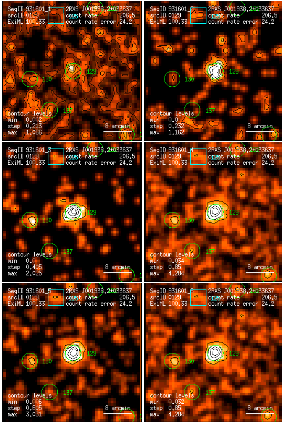
Figure 129: RASS 931601: detection 0129: band rate images, Gaussian filter: (1) PSPC channels 11 – 41, (2) 52 – 90, (3) 91 – 201, (4) 11 – 235, (5) 52 – 201, (6) 11 – 201. Broad band rates in counts/ks. Band rate contour levels in counts/ks/arcmin 2 .
