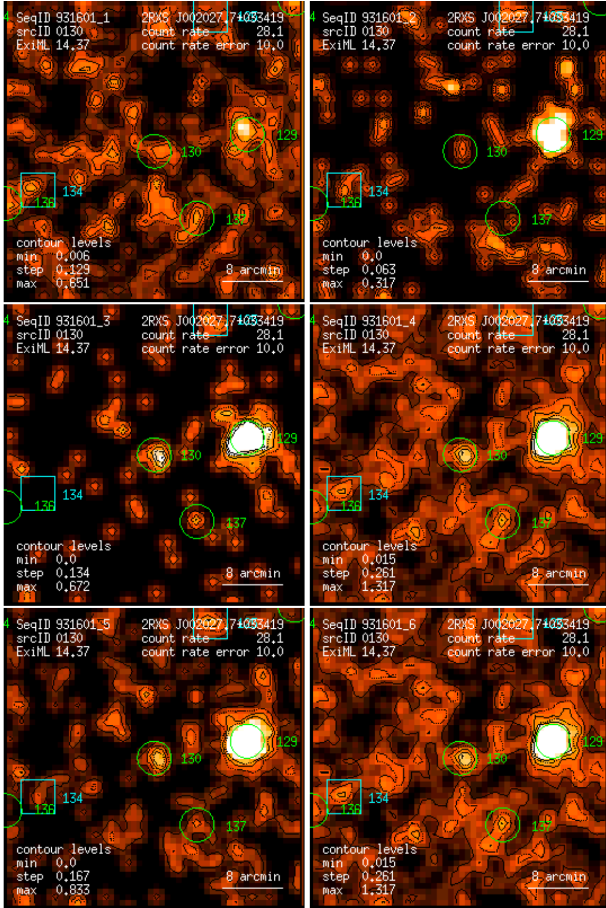
Figure 130: RASS 931601: detection 0130: band rate images, Gaussian filter: (1) PSPC channels 11 – 41, (2) 52 – 90, (3) 91 – 201, (4) 11 – 235, (5) 52 – 201, (6) 11 – 201. Broad band rates in counts/ks. Band rate contour levels in counts/ks/arcmin 2 .
