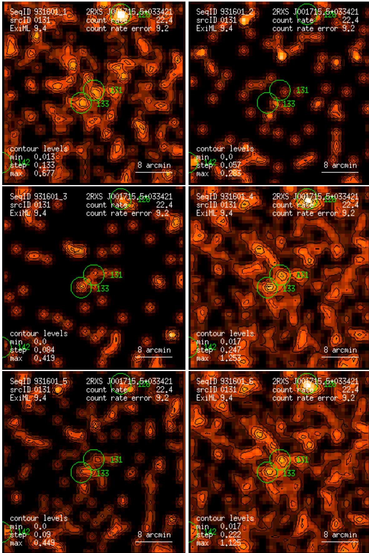
Figure 131: RASS 931601: detection 0131: band rate images, Gaussian filter: (1) PSPC channels 11 – 41, (2) 52 – 90, (3) 91 – 201, (4) 11 – 235, (5) 52 – 201, (6) 11 – 201. Broad band rates in counts/ks. Band rate contour levels in counts/ks/arcmin 2 .
