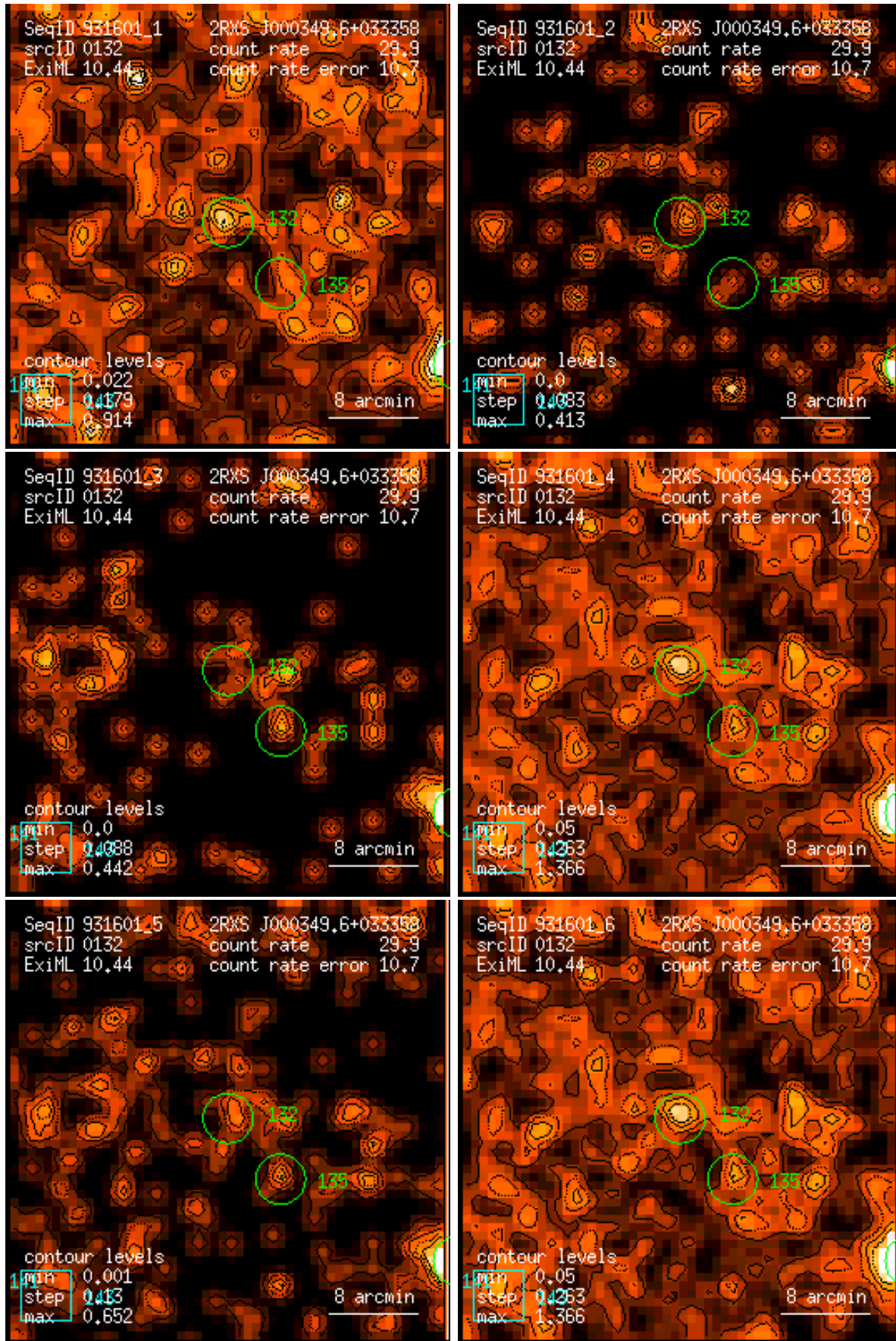
Figure 132: RASS 931601: detection 0132: band rate images, Gaussian filter: (1) PSPC channels 11 – 41, (2) 52 – 90, (3) 91 – 201, (4) 11 – 235, (5) 52 – 201, (6) 11 – 201. Broad band rates in counts/ks. Band rate contour levels in counts/ks/arcmin 2 .
